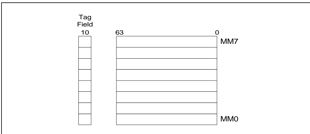
Figure 2-7. MMX™ Register Set
