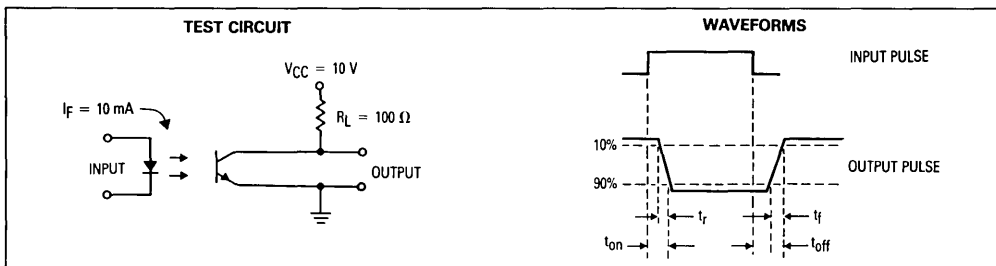
Figure 11. Switching Times
