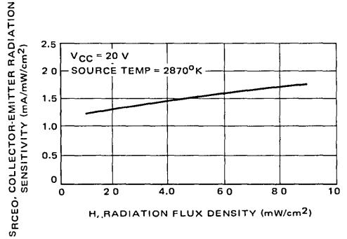
FIGURE 14 — Open Base Sensitivity versus Radiation for MRD300
