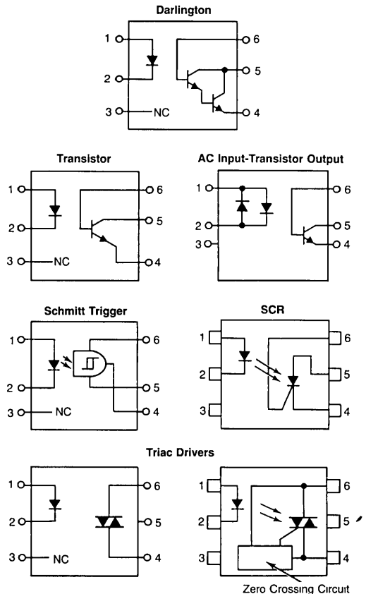
Figure 6. Various Optoisolator Configurations
