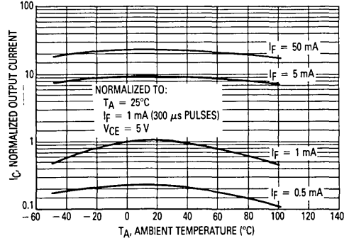
Figure 2. Output Current versus Temperature
