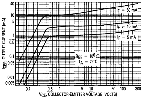
Figure 3. Output Characteristics
