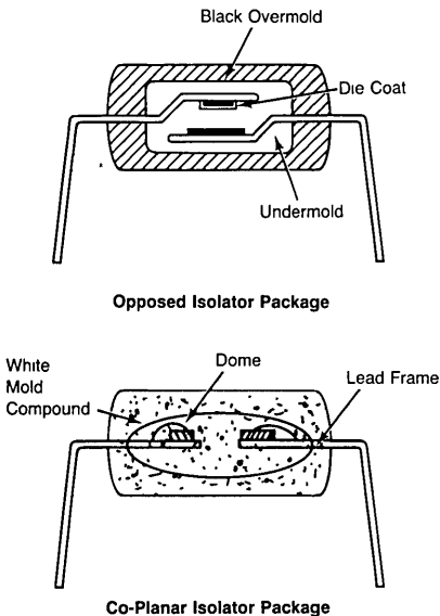
Figure 5. Geometric Designs for Optoisolators
