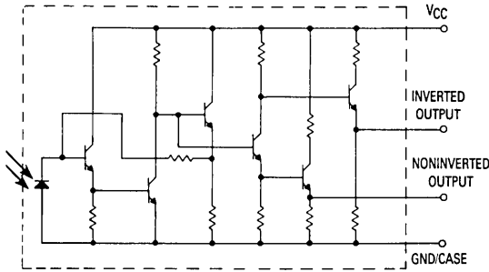
Figure 1. Equivalent Schematic
