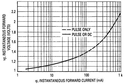
Figure 2. Forward Characteristics
