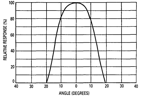
Figure 8. Angular Response
