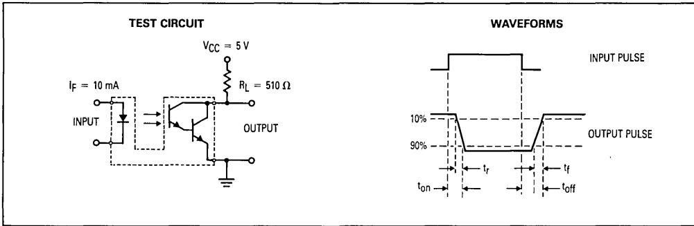
Figure 9. Switching Times
