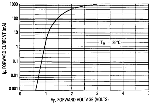
Figure 1. Forward Current versus LED Forward Voltage
