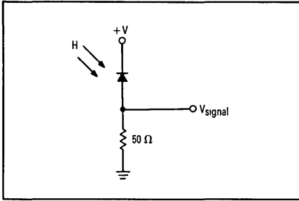
Figure 1. Operating Circuit
