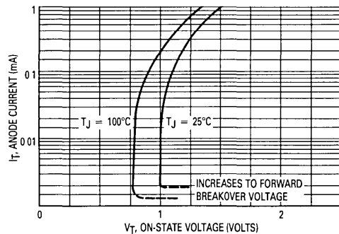
Figure 2. On-State Characteristics
