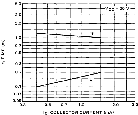
FIGURE 22 – Switching Storage and Fall Times for MRD300
