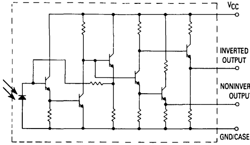
Figure 1. Equivalent Schematic
