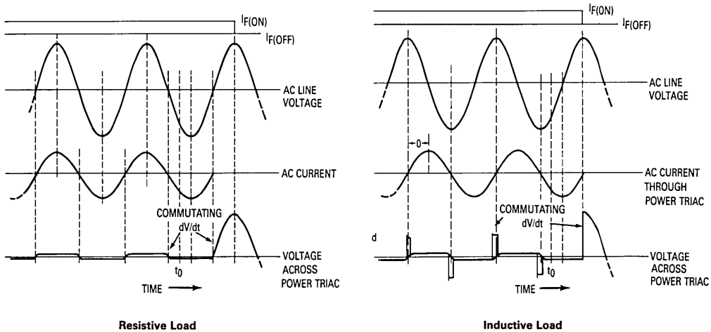
Figure 12. Current and Voltage Waveforms During Commutation
