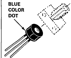
CASE 366-01 PLASTIC
