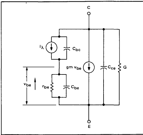
FIGURE 3 – Floating Base Approximate Model of Phototransistor
