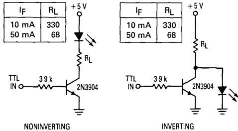
Figure 11. TTL Transmitters
