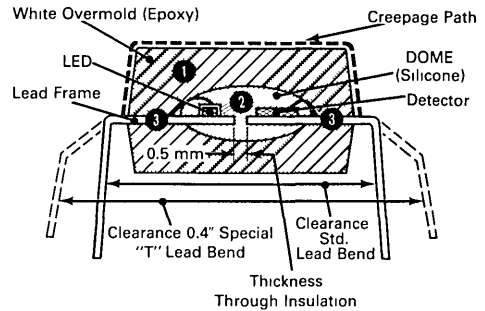
Figure 1. "DOME" Package
