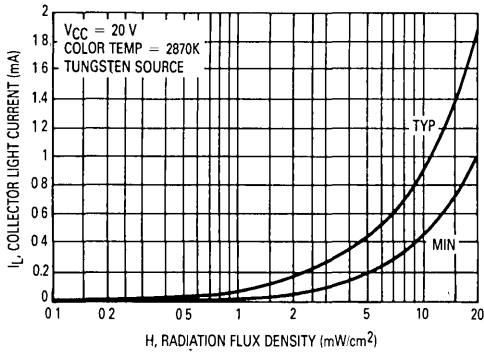
Figure 1. Collector-Emitter Sensitivity
