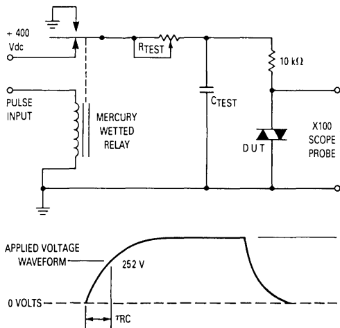
Figure 7. Static dv/dt Test Circuit
