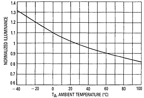
Figure 2. Illuminance versus Temperature
