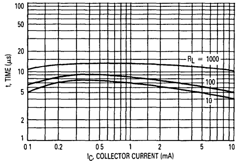
Figure 4. Typical Turn-Off Switching Times
