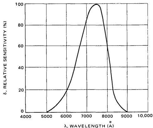
FIGURE 2 – Spectral Response of Cadmium Selenide
