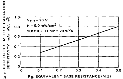
FIGURE 15 — Effect of Base Resistance on Sensitivity of MRD300
