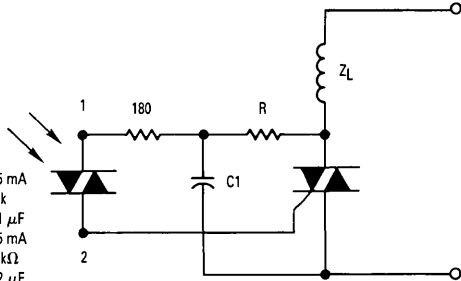
Figure 8. Inductive Load
