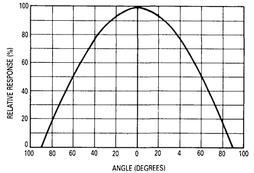
Figure 6. Angular Response
