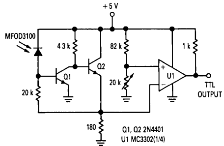
Figure 14. 1 MHz Pin Receiver
