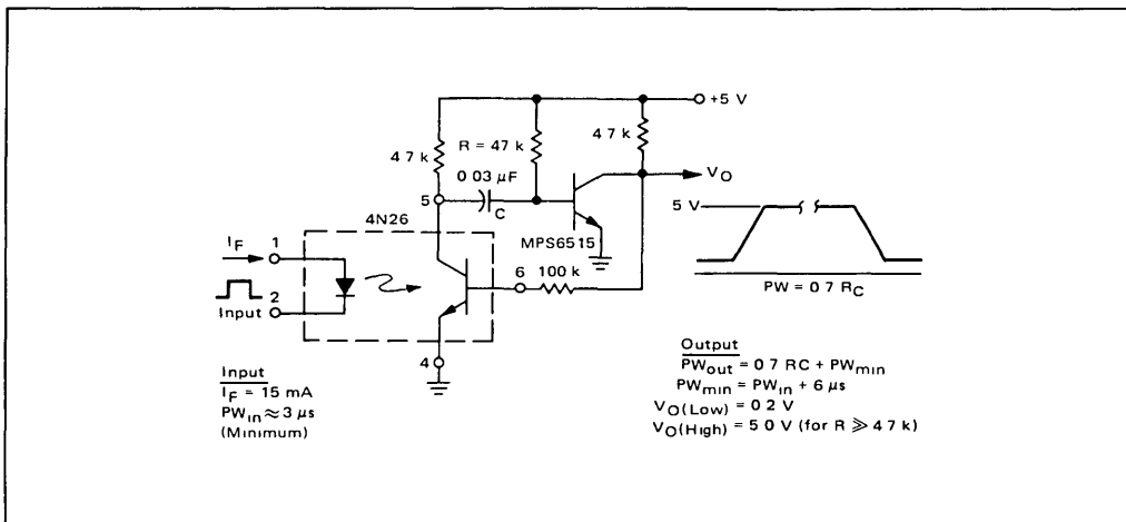
FIGURE 15 – Pulse Stretcher
