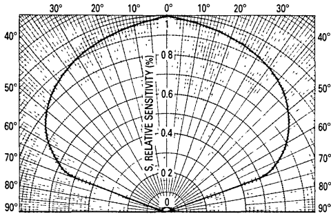
Figure 3. Angular Response
