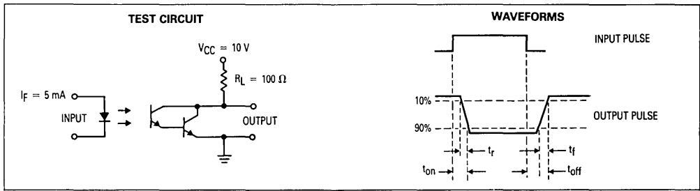
Figure 9. Switching Times
