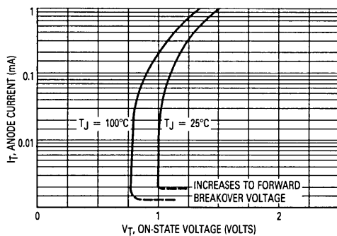
Figure 2. On-State Characteristics
