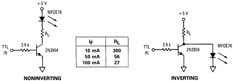
Figure 6. TTL Transmitters
