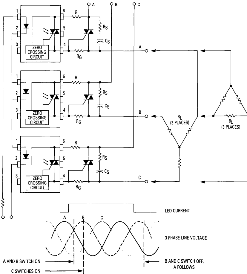
Figure 16. 3 Phase Control Circuit
