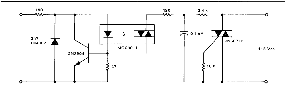
FIGURE 10 — Solid-State Relay
