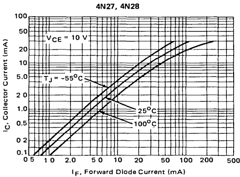
FIGURE 4B – DC Current Transfer Ratio
