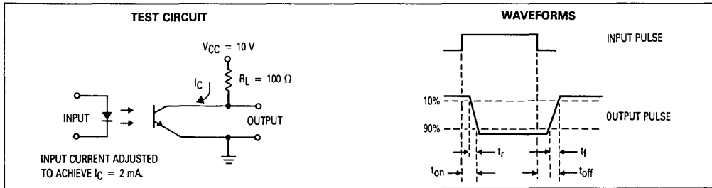
Figure 10. Switching Times
