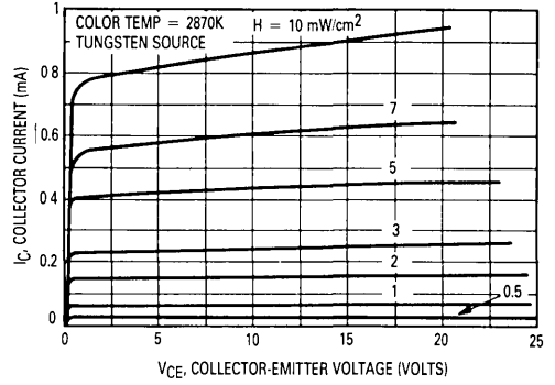
Figure 2. Collector-Emitter Characteristics
