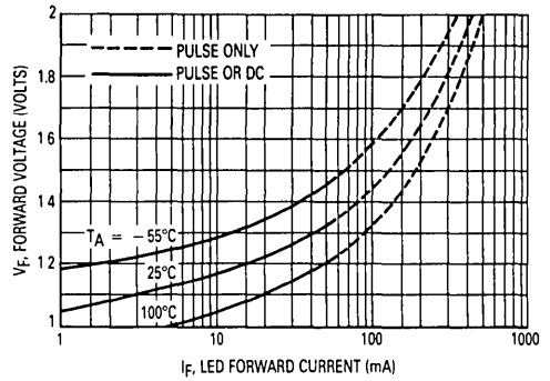
Figure 4. Forward Characteristics
