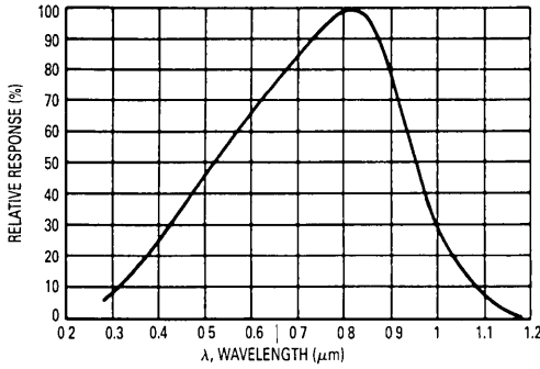
Figure 1. Relative Spectral Response
