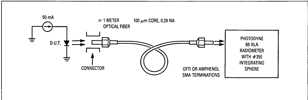
Figure 6. Coupling Efficiency
