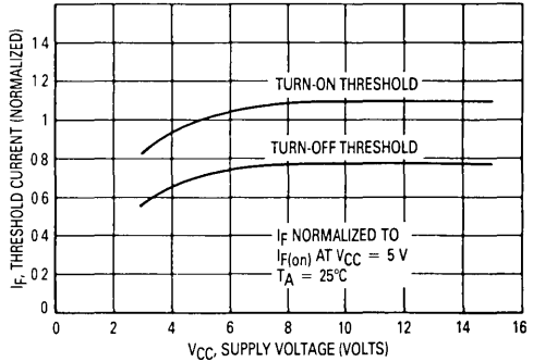
Figure 6. Threshold Current versus Supply Voltage
