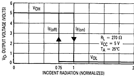
Figure 2. Transfer Characteristics
