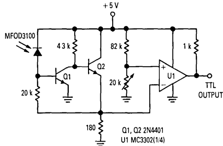
Figure 12. 1 MHz PIN Receiver
