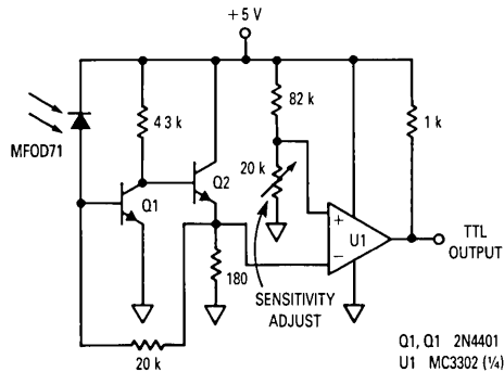
Figure 7. TTL Receiver
