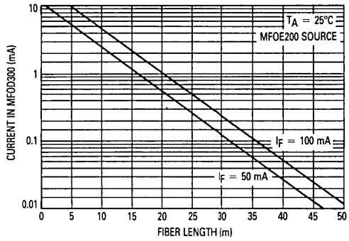
Figure 2. Coupled System Performance versus Fiber Length
