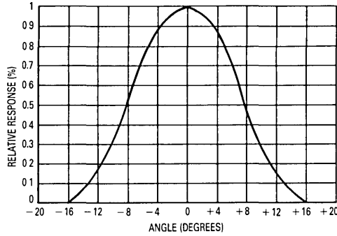
Figure 7. Angular Response
