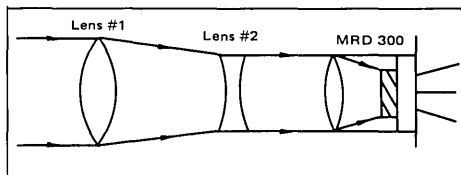
FIGURE 14 – Effective Use of External Optics with the MRD 300
