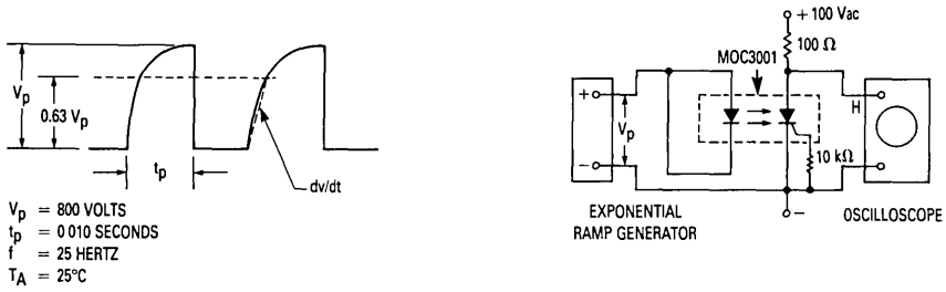
Figure 8. Coupled dv/dt — Test Circuit
