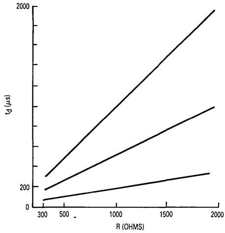
Figure 9. Time Delay t_d versus Current Limiting Resistor R
