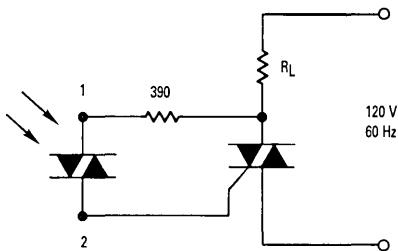
Figure 7. Resistive Load
