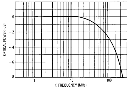
Figure 8. Typical LED Bandwidth
