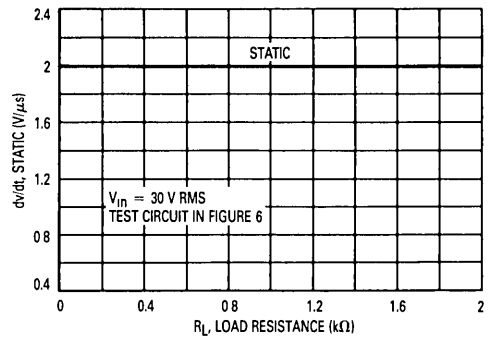
Figure 3. dv/dt versus Load Resistance
