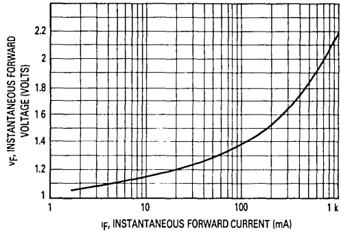
Figure 2. Forward Characteristics
