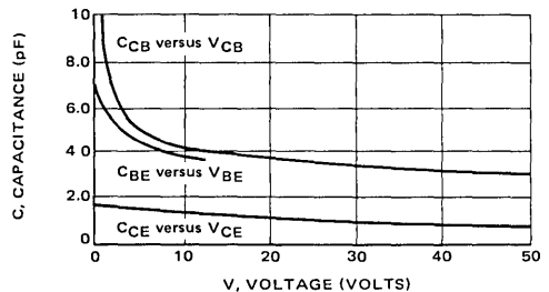
FIGURE 16 — Junction Capacitances versus Voltage for MRD300
