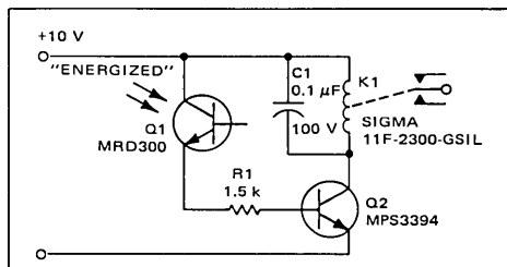
FIGURE 25 – Light-Operated Relay
