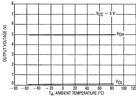
Figure 8. Output Voltage versus Ambient Temperature
