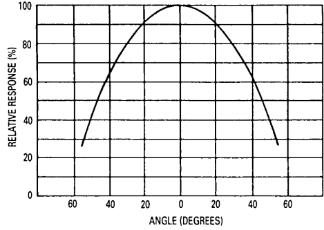
Figure 2. Angular Response
