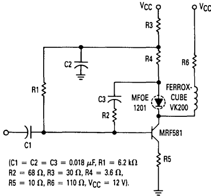
Figure 11. LED Drive Circuit to 100 MHz
