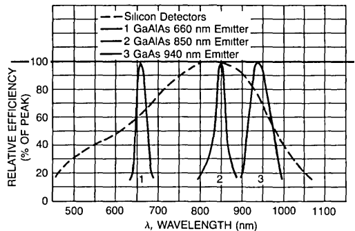
Figure 2. Emissivity versus Wavelength
