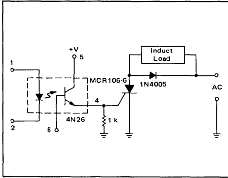
FIGURE 11 – Coupler-Driven SCR
