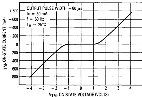
Figure 1. On-State Characteristics
