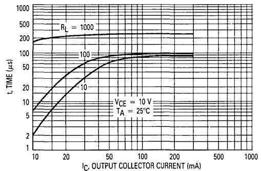
Figure 6. Typical Turn-Off Switching Times
