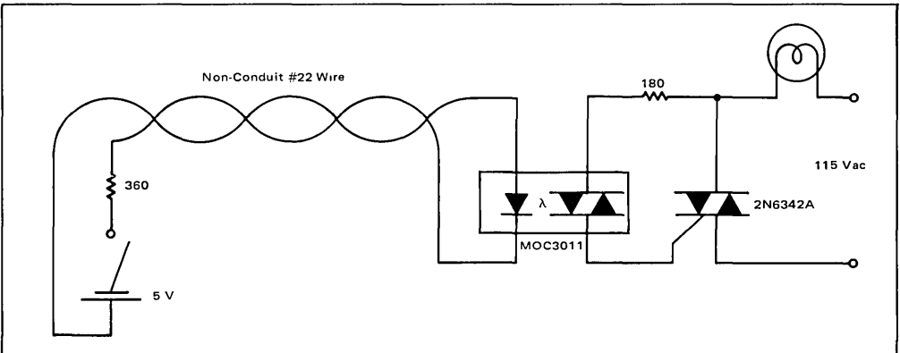
FIGURE 9 – Remote Control of ac Loads Through Low Voltage Non-Conduct Cable
