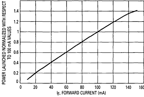
Figure 1. Normalized Power Launched versus Forward Current
