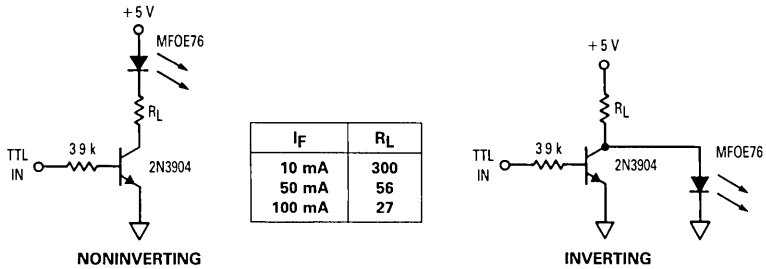
Figure 6. TTL Transmitters
