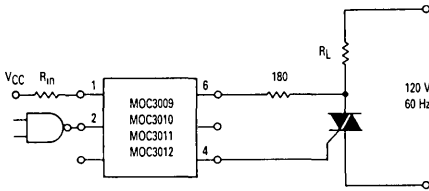
Figure 8. Resistive Load
