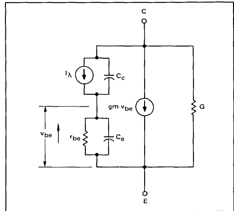
FIGURE 8 – Floating Base Approximate Model of Phototransistor
