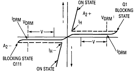
Figure 3. Triac Voltage-Current Characteristic
