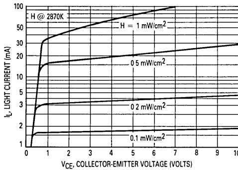
Figure 3. Collector Characteristics
