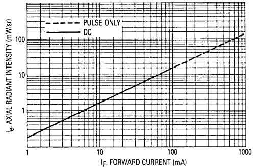
Figure 4. Intensity versus Forward Current
