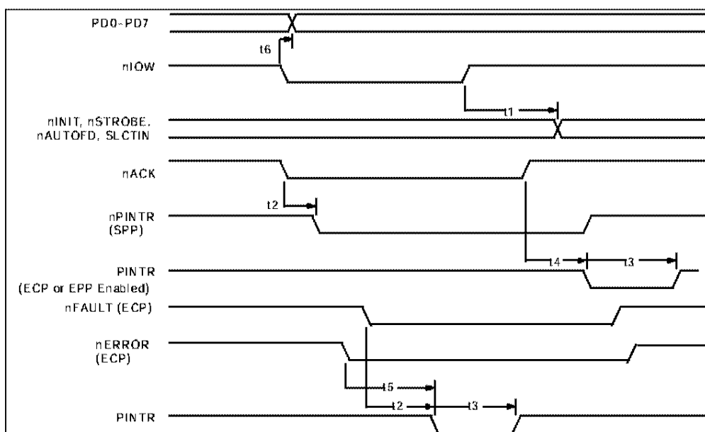
FIGURE 12 - PARALLEL PORT TIMING
