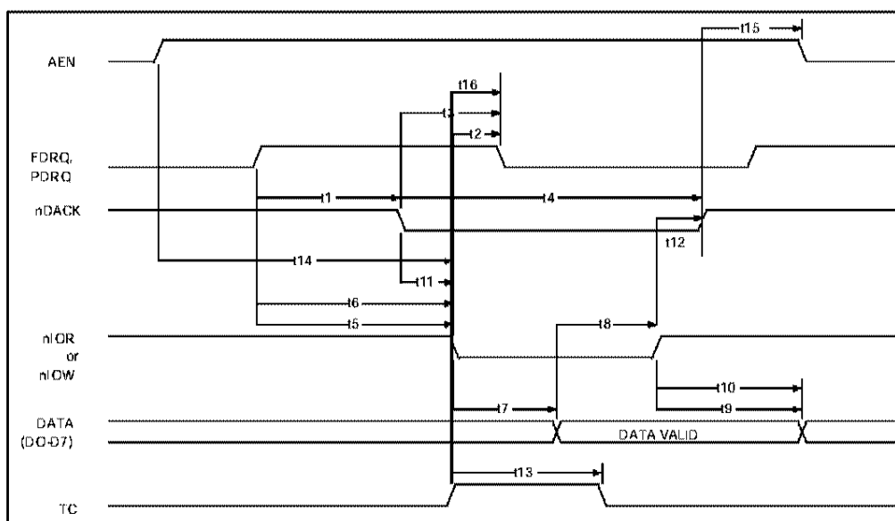
FIGURE 9A - DMA TIMING (SINGLE TRANSFER MODE)
