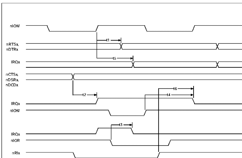
FIGURE 11 - SERIAL PORT TIMING
