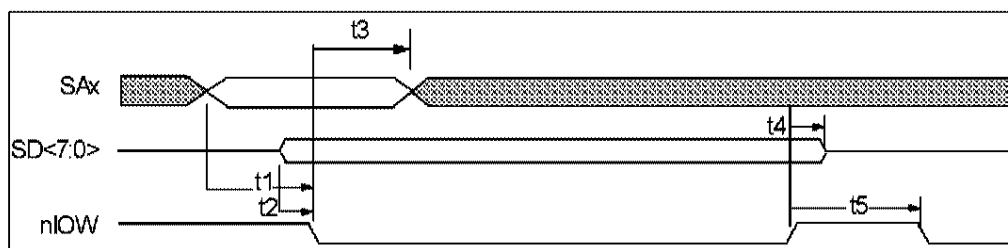
FIGURE 3 - IOW TIMING FOR PORT 92
