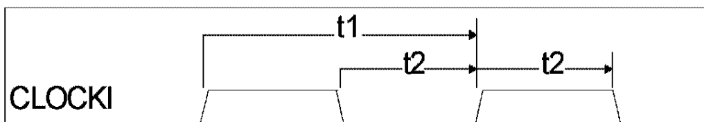
FIGURE 8A - INPUT CLOCK TIMING
