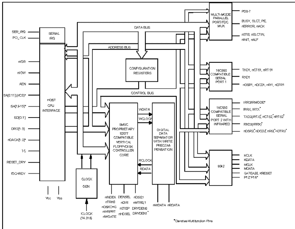
FIGURE 1 - FDC37M61x BLOCK DIAGRAM
