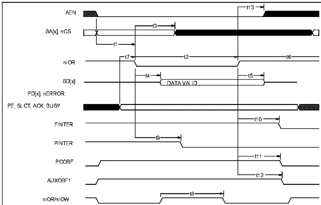
FIGURE 6 - ISA READ
