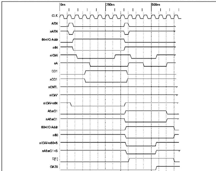
Gate A20 Turn-On Sequence Timing
