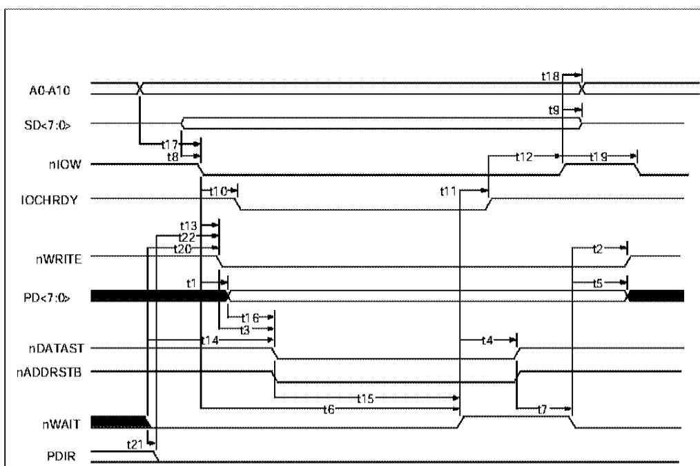
FIGURE 13A - EPP 1.9 DATA OR ADDRESS WRITE CYCLE
