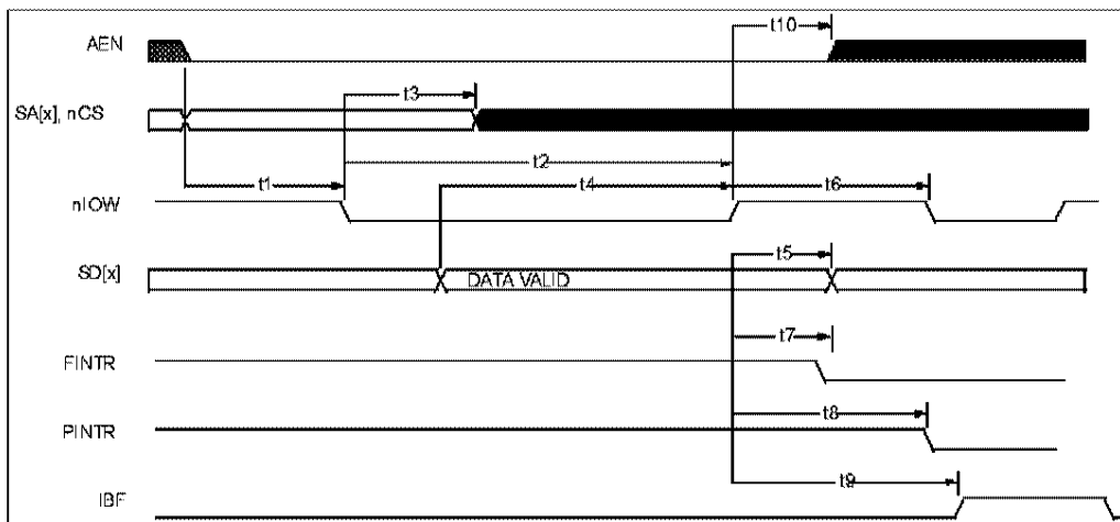
FIGURE 5 - ISA WRITE
