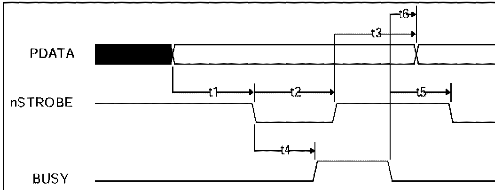
FIGURE 17 - PARALLEL PORT FIFO TIMING
