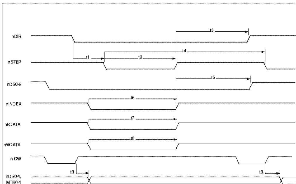
FIGURE 10 - DISK DRIVE TIMING (AT MODE ONLY)
