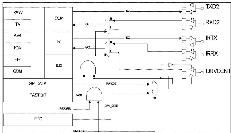
FIGURE 2 - IR INTERFACE BLOCK DIAGRAM
