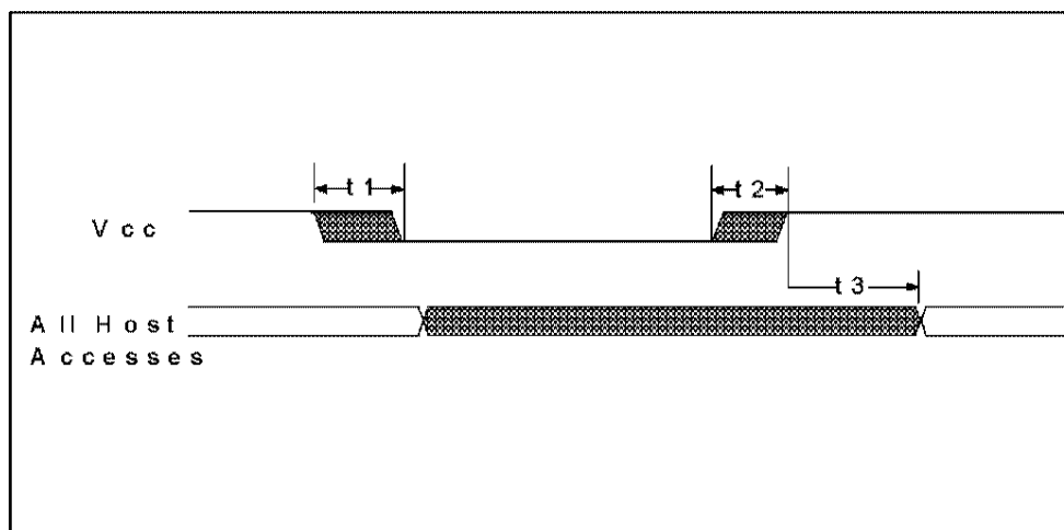
FIGURE 4 - POWER-UP TIMING
