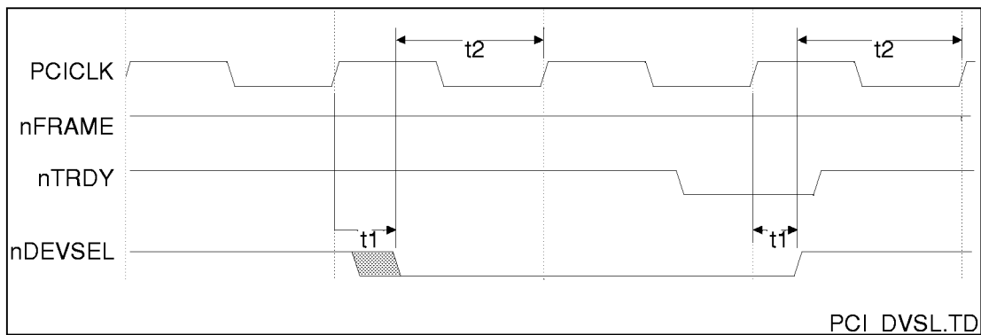
FIGURE 7 - PCI/nDEVSEL TIMING
