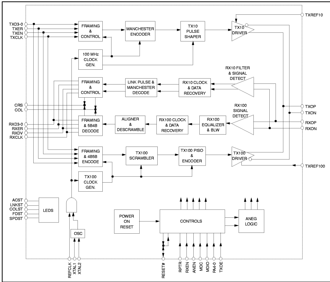
FIGURE 2 – LAN83C180 BLOCK DIAGRAM
