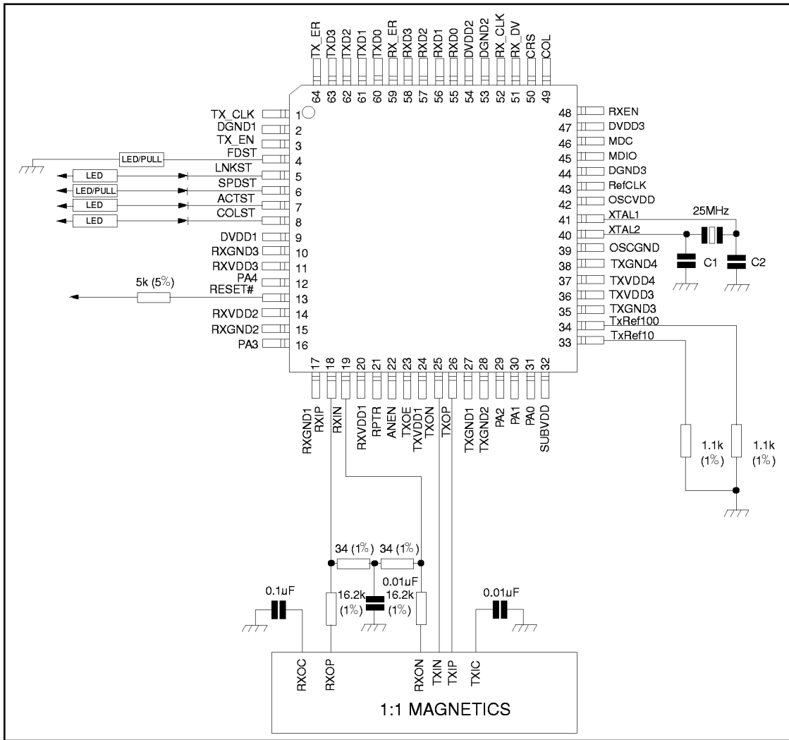
FIGURE 3 - EXTERNAL COMPONENTS
