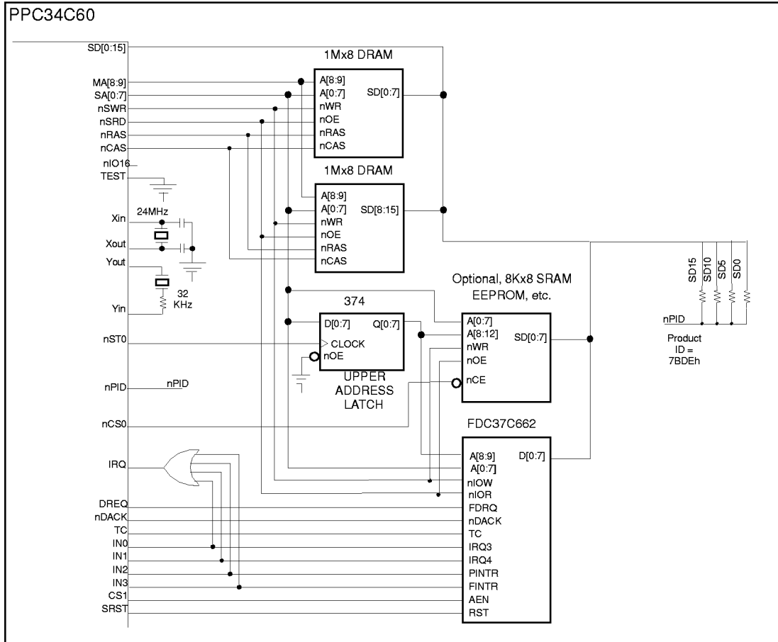
FIGURE 3 – TYPICAL SYSTEM INTERFACE
