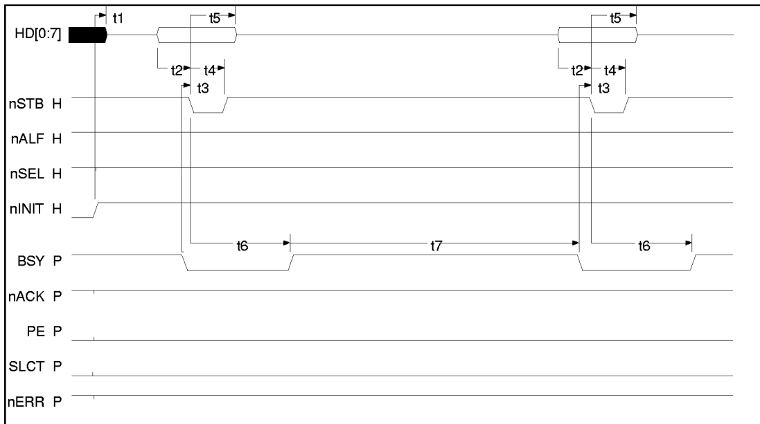
FIGURE 12 - SPP DATA WRITE TIMING (PARALLEL PORT SIGNALS)
