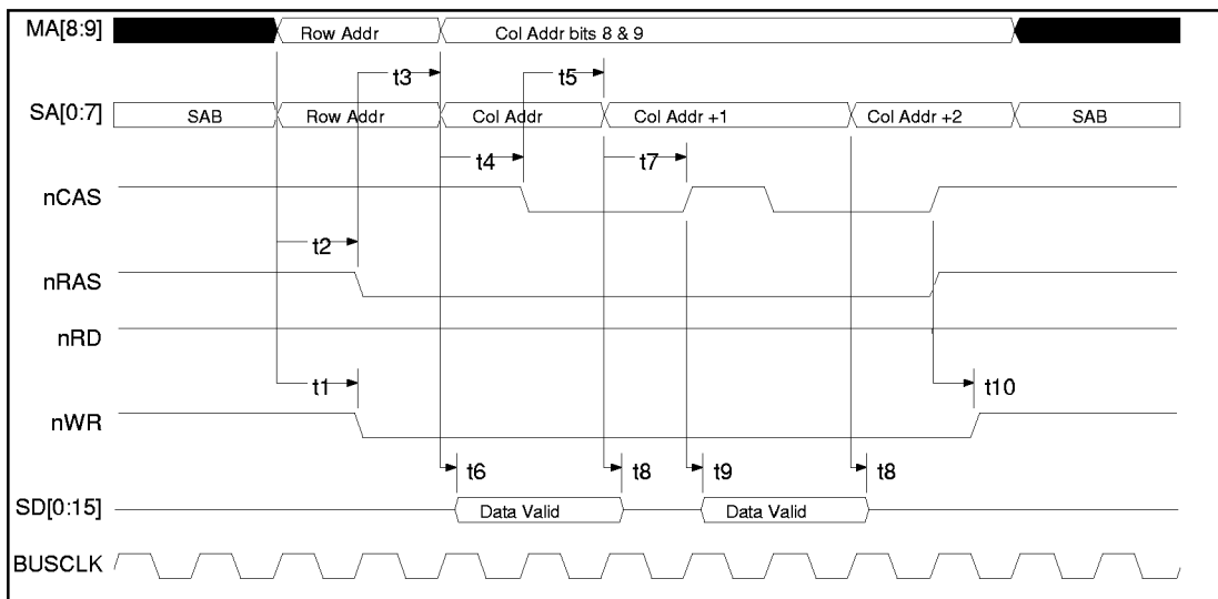
FIGURE 24 - DRAM WRITE CYCLE TIMING
