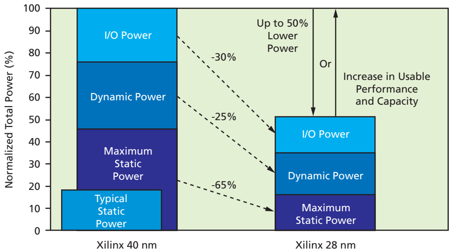
Figure 2 – Xilinx 7 series FPGAs consume half the power of devices built in the earlier 40-nm process.
