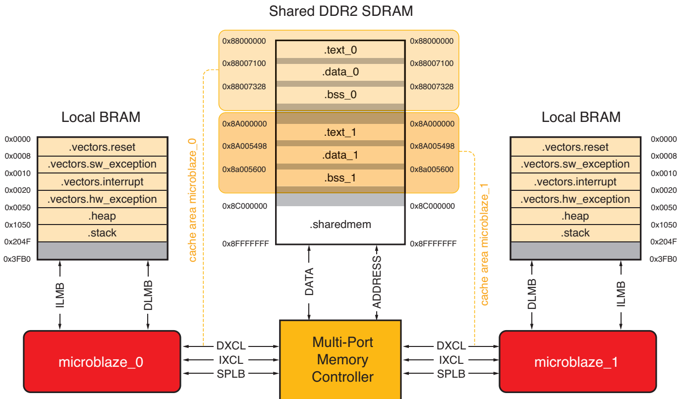
Figure 2 – Memory map of the DMX system
