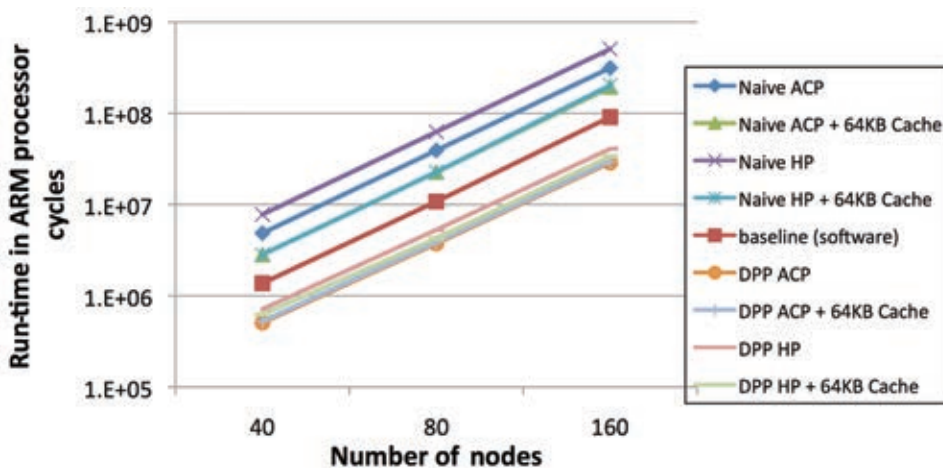
Figure 9 – Run-time comparison for Floyd-Warshall algorithm
