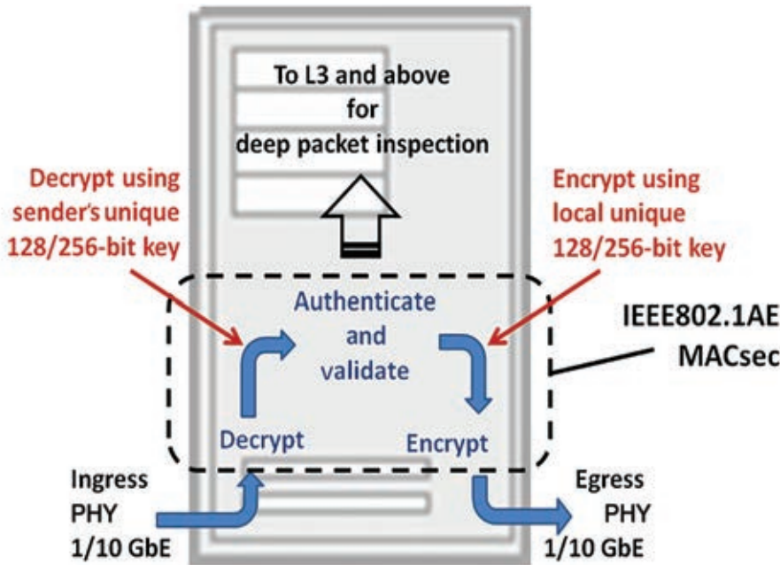
Figure 2 – The message is decrypted on the ingress port and encrypted on the egress port.
