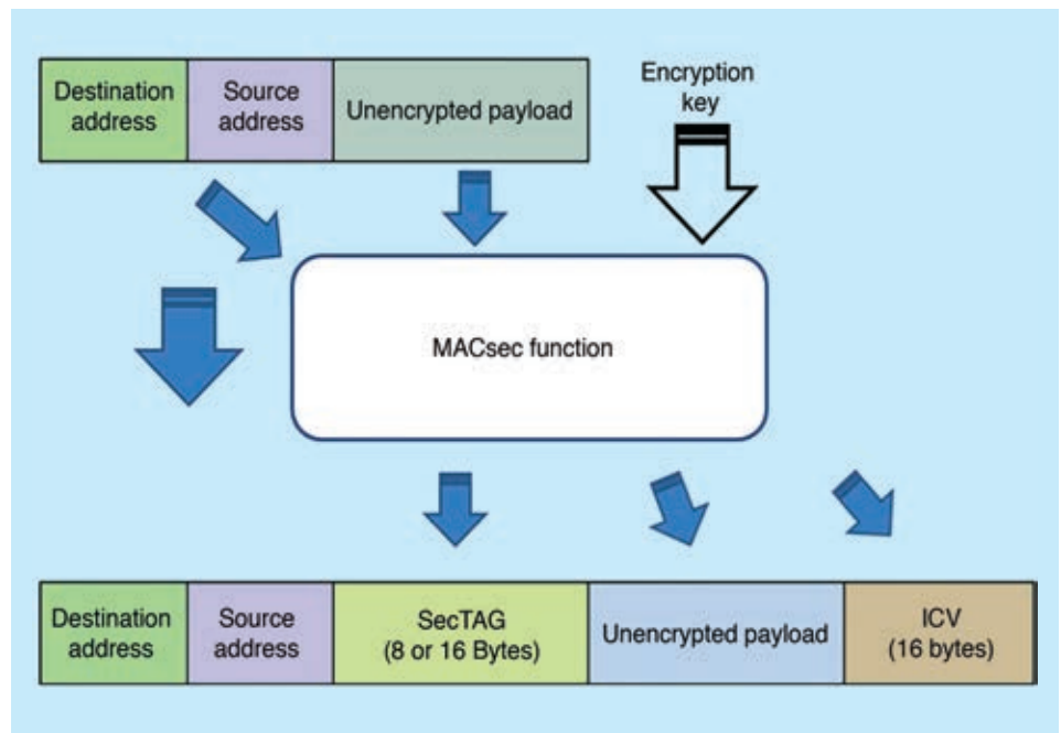
Figure 3 – The MACsec frame structure includes a field known as the MAC Security TAG (SecTAG), which defines the EtherType and flags whether the packet is encrypted.
