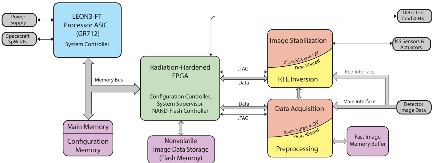
Figure 2 – Architecture of the PHI data-processing unit
