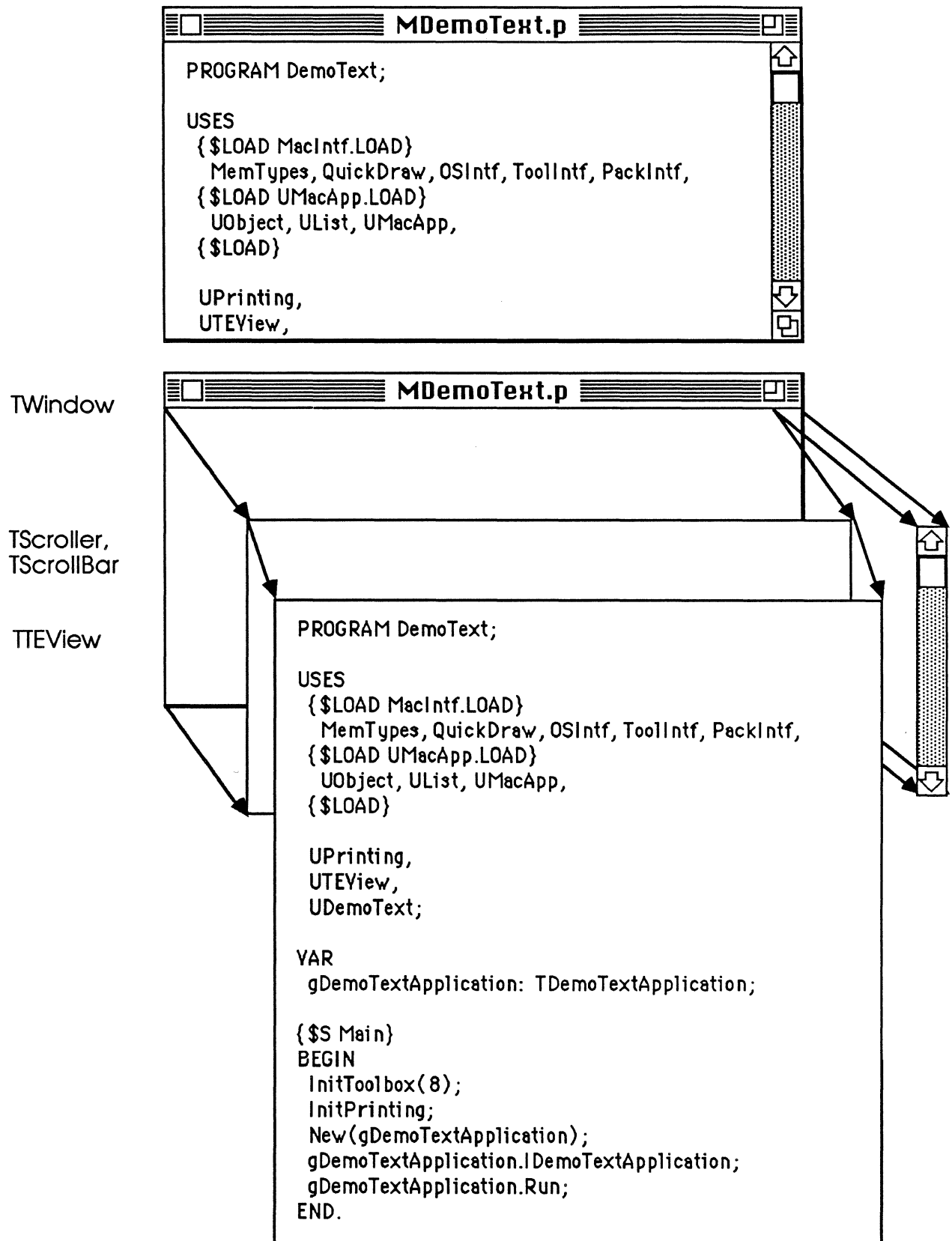
Figure 2: New MacApp Display Architecture
