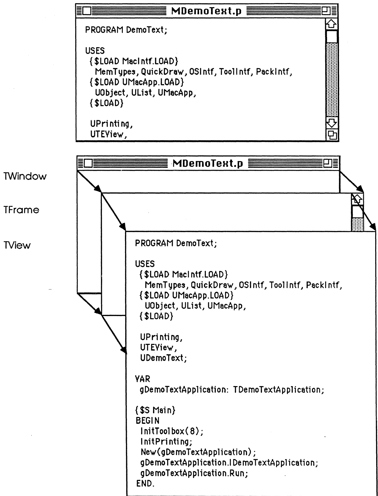
Figure 1: Old MacApp Display Architecture
