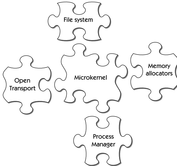
FIGURE 2.3 The microkernel and other modularized reentrant services
