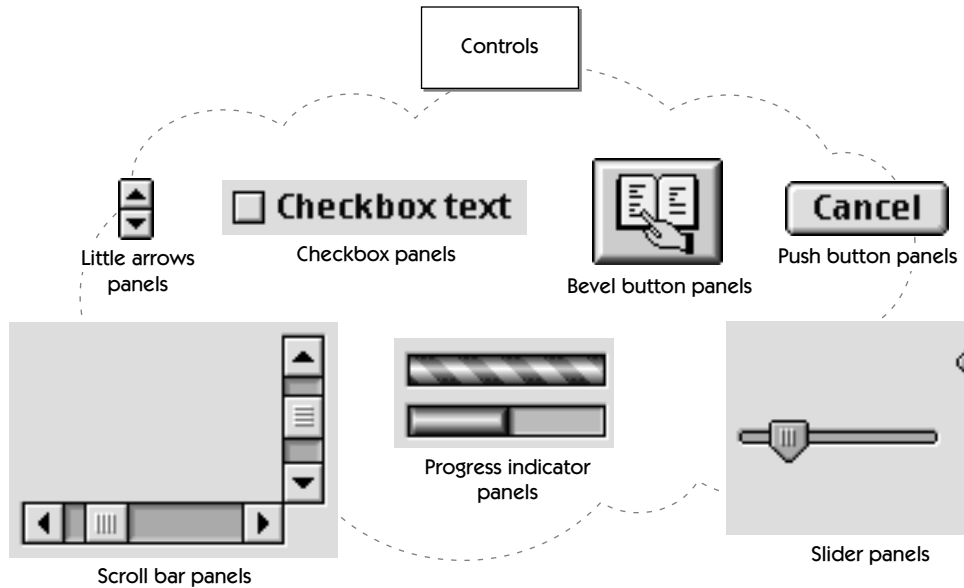
FIGURE 12.14 Examples of controls derived from subclasses of the controls class
