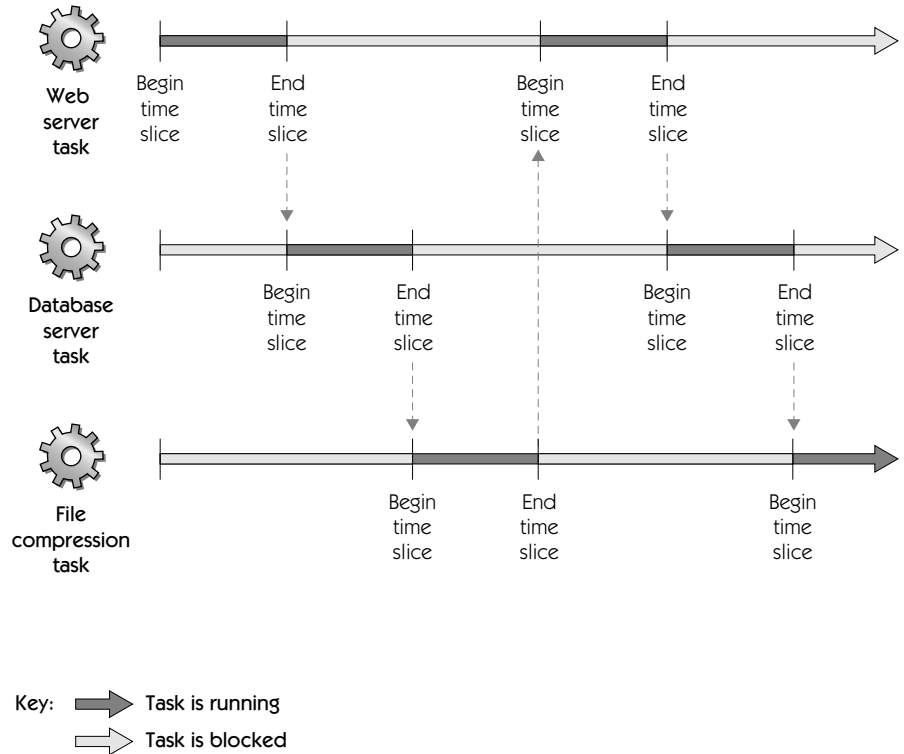
FIGURE 4.6 Execution time divided by time slices for tasks with equal priority
