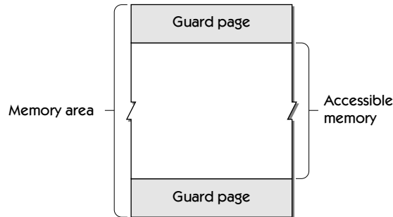
FIGURE 3.5 A memory area with guard pages
