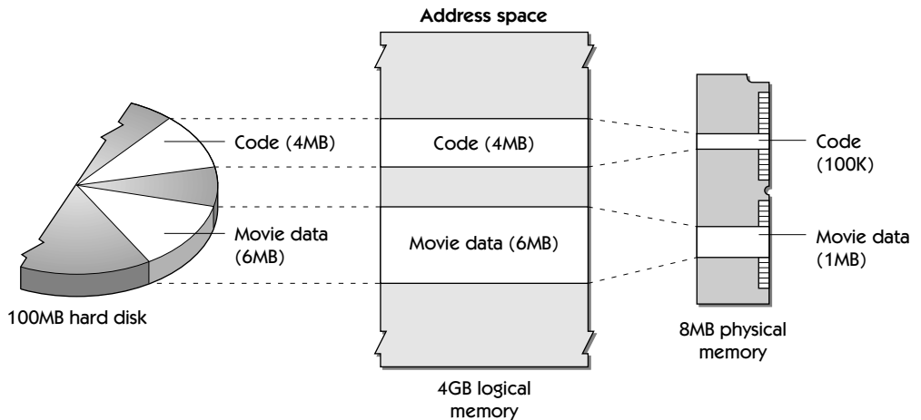
FIGURE 6.1 The association of disk files, memory areas, and physical memory
