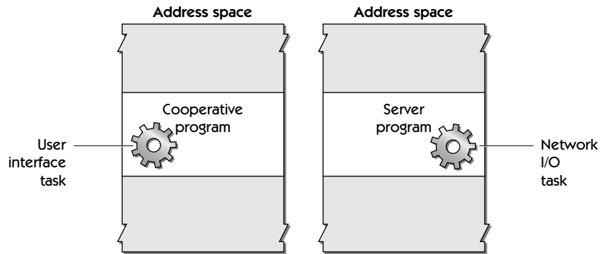
FIGURE 5.1 Tasks in two separate processes
