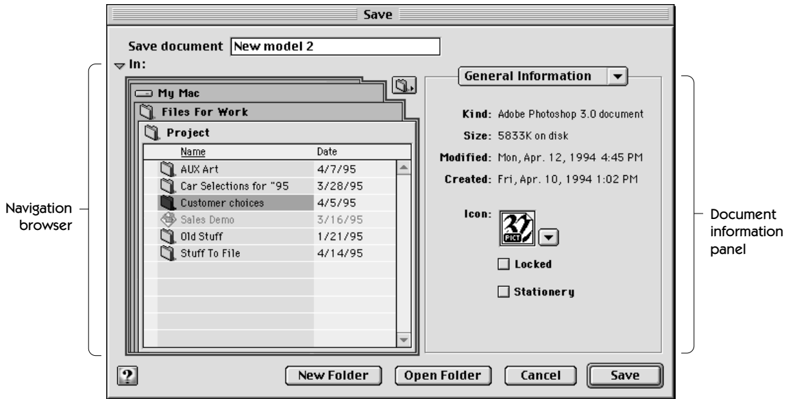
FIGURE 10.1 Standard navigation browser and the general information panel
