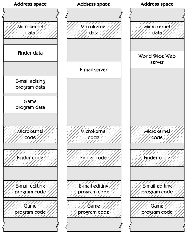
FIGURE 3.4 System-wide memory areas
