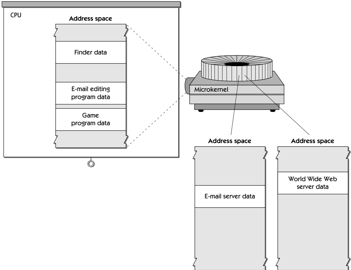
FIGURE 3.3 Switching between address spaces
