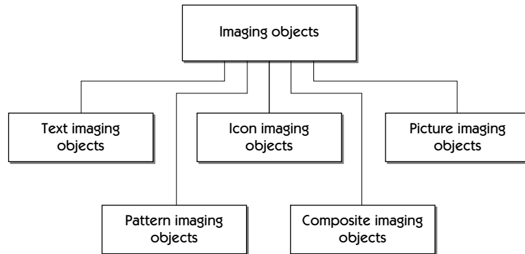
FIGURE 12.17 The inheritance hierarchy for the imaging objects class library
