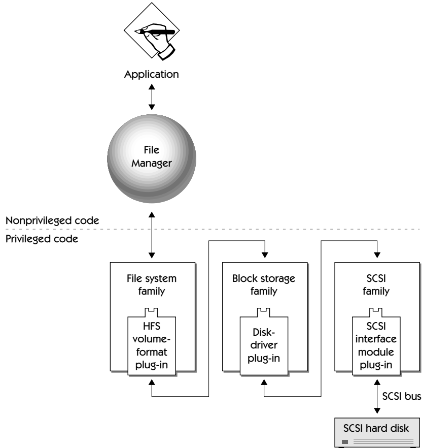
FIGURE 11.1 Interactions between an application saving a file and several I/O families
