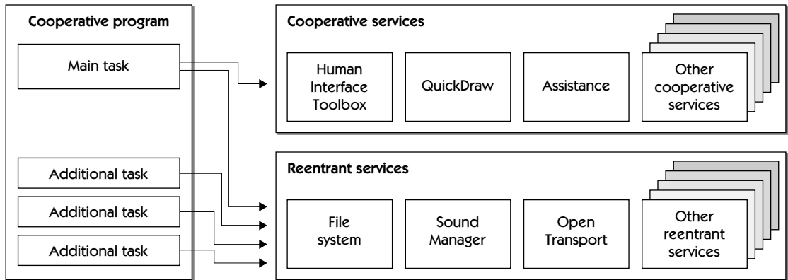
FIGURE 4.7 Making all calls to cooperative services from the main task of a cooperative program
