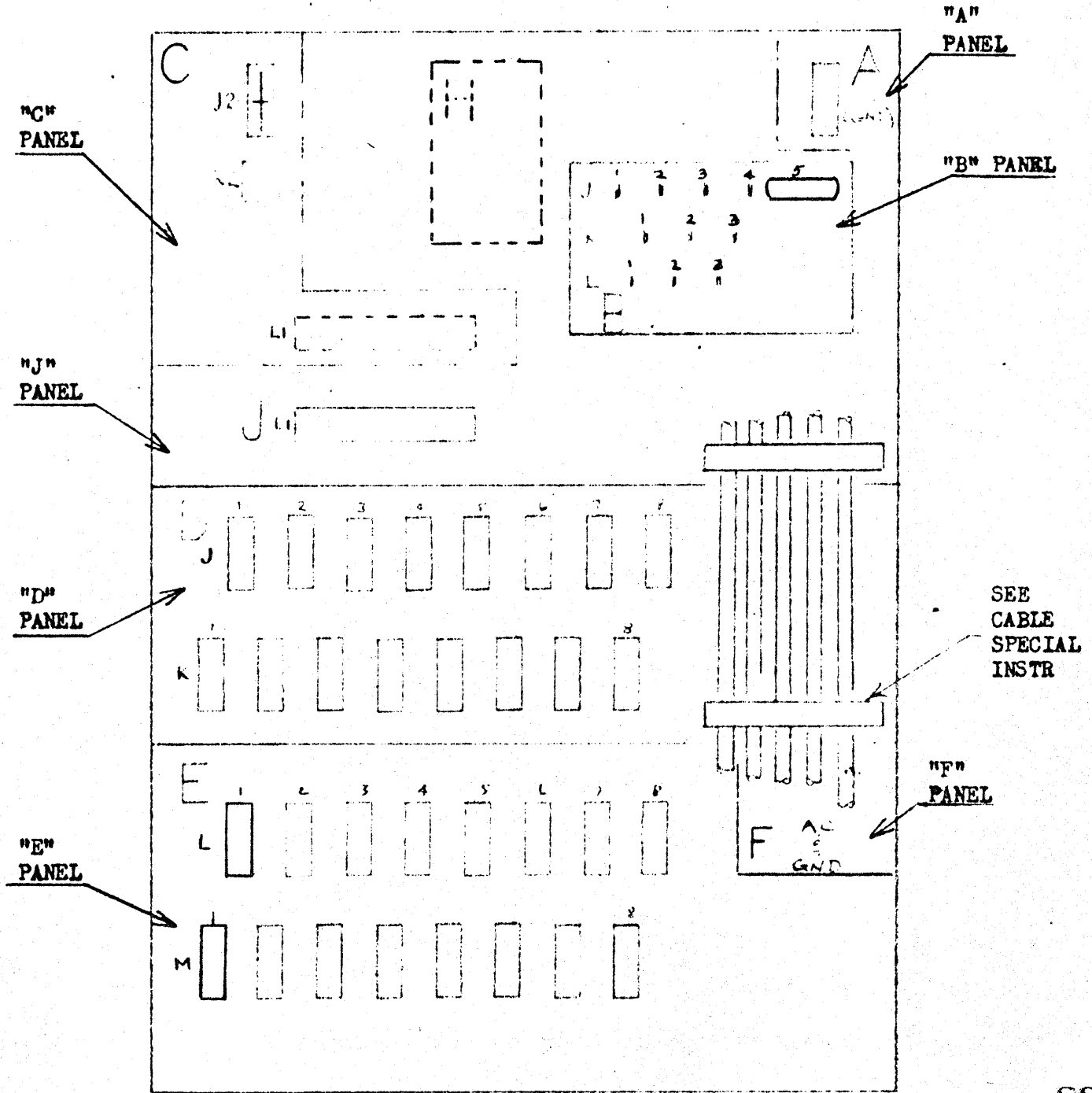
D Rack--Rear View
