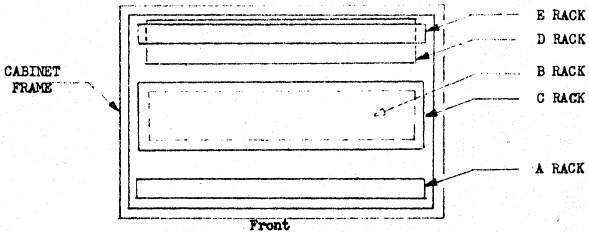
RACK LOCATIONS---Top View of Cabinet
