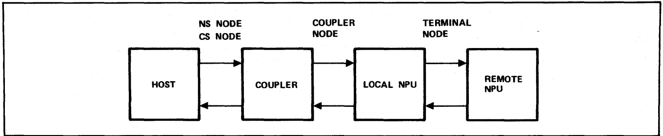
Figure 2-6. Sample Logical Link Connections (Shown for Local and Remote NPUs)
