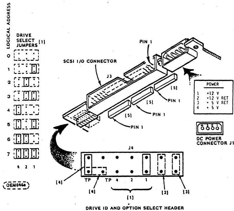
FIGURE 11.1-1. WREN V SCSI DRIVE ID AND OPTION SELECT HEADER
