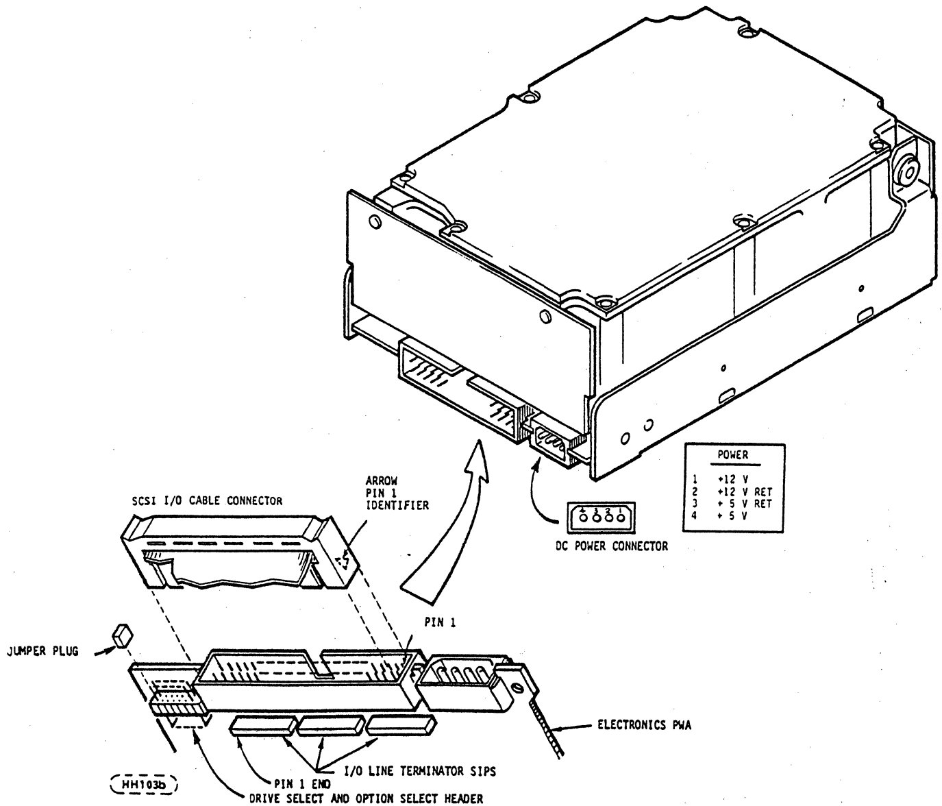
FIGURE 10.3-3. I/O CONNECTION
