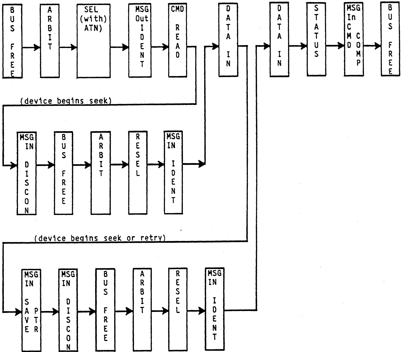
FIGURE 13.3-2. DISCONNECT EXAMPLE
