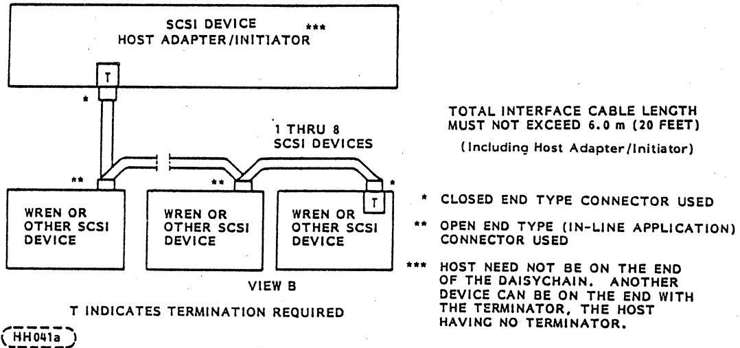
FIGURE 10.3-2. INTERFACE CABLING
