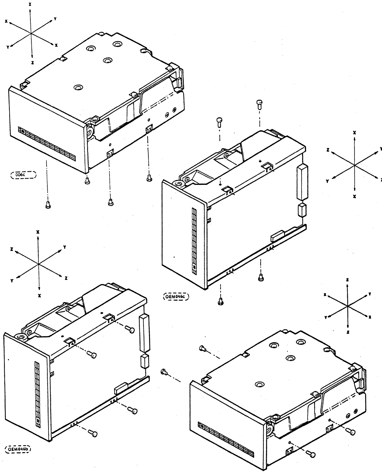
FIGURE 7.4-1. RECOMMENDED MOUNTING
