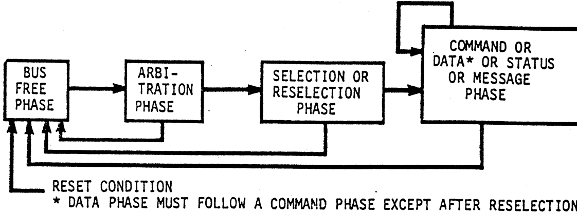
FIGURE 12.3-2. PHASE SEQUENCES WITH ARBITRATION
