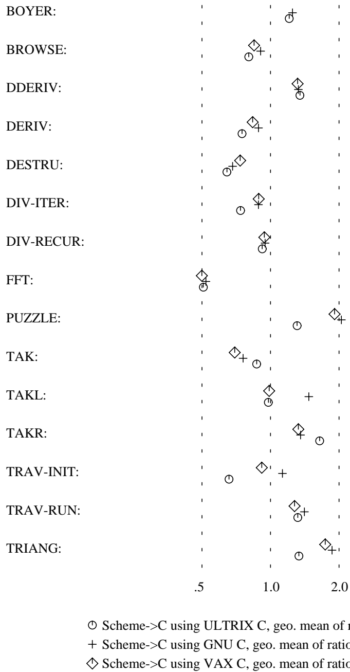
Figure 1: Performance of Scheme->C relative to VAX Common Lisp V2.2
