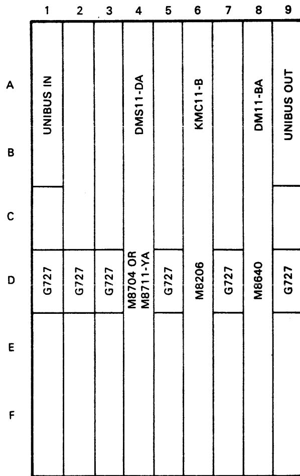
Figure 2-9 DD11-DK Nine-Slot Backplane with KMC11-B Board Locations (Viewed from the Backplane Pin-Side)
