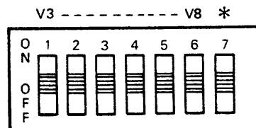
Figure 2-7 KMC11-B (M8206 - Etch Rev D) UNIBUS Microprocessor Address Selection Switch E129
