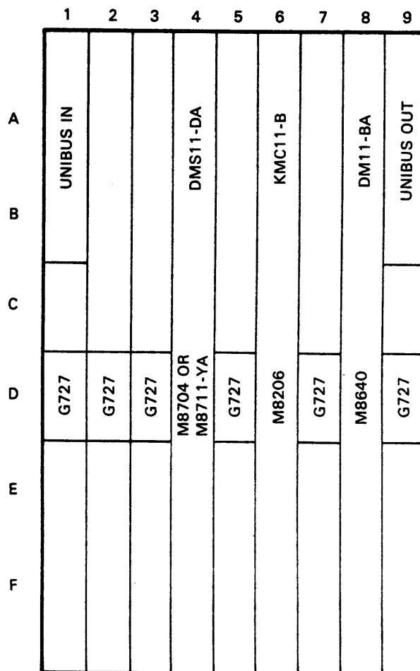
Figure 2-1 KMC11-B Microprocessor Placement in a Nine-Slot Expansion Box
