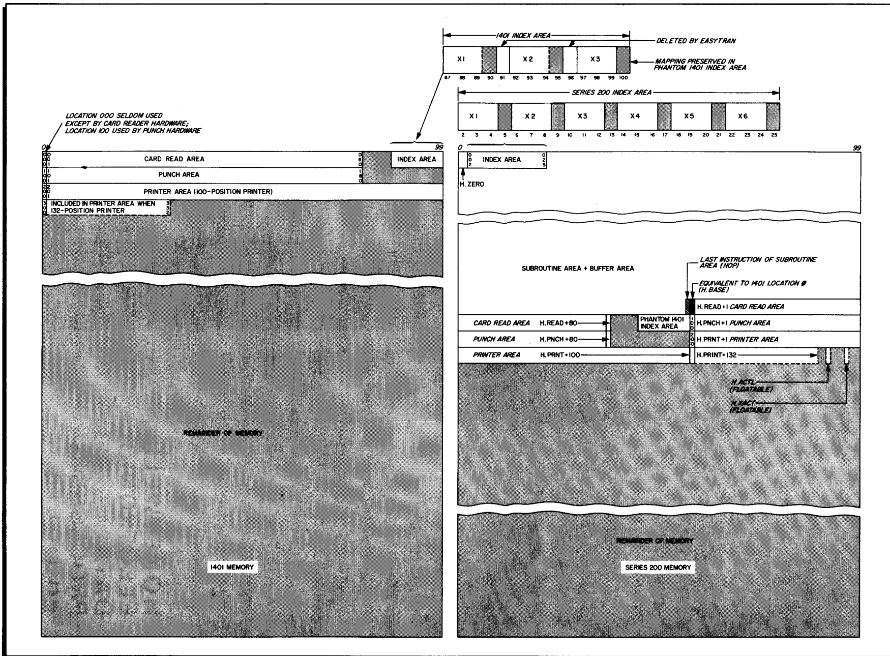
Figure 2-1. Easytran Memory Mapping
