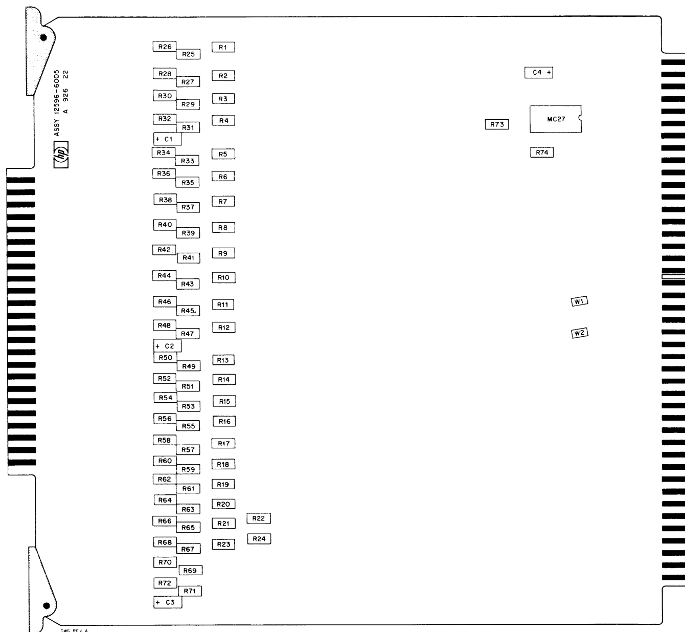
Figure 3-7. I/O-X2 Extender Card (12596-6005) Parts Location Diagram
