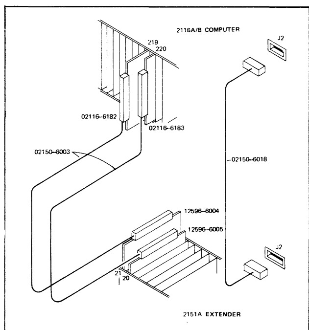
Figure 1-1. HP 12596A I/O Extender Interface Kit Installation
