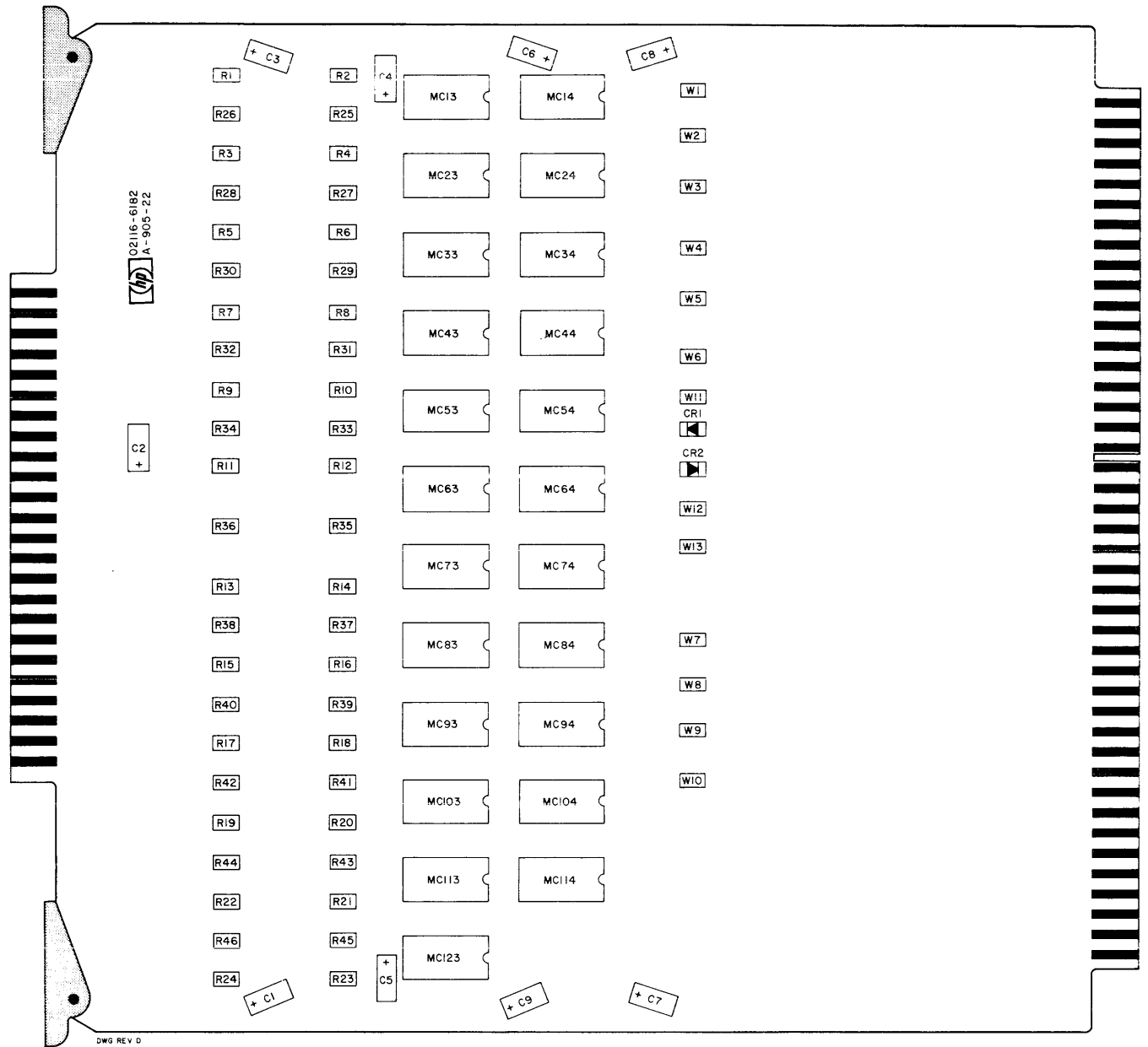
Figure 3-1. I/O-1 Extender Driver Card (02116-6182) Parts Location Diagram
