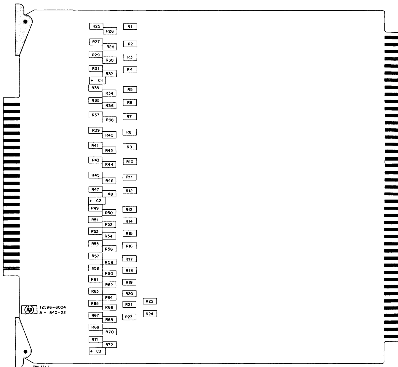
Figure 3-5. I/O-X1 Extender Card (12596-6004) Parts Location Diagram
