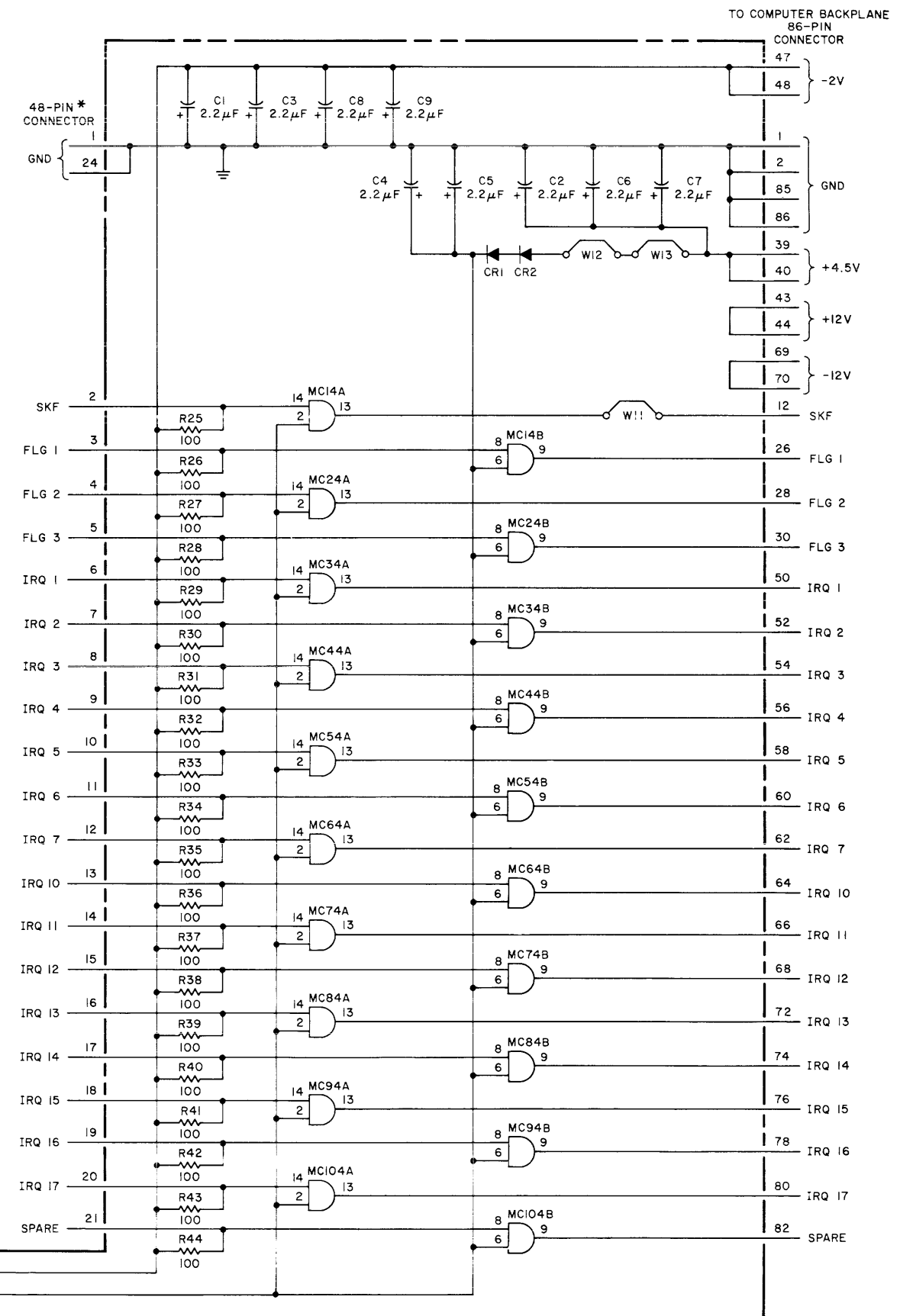
Figure 3-2. I/O-1 Extender Driver Card (02116-6182) Schematic Diagram
