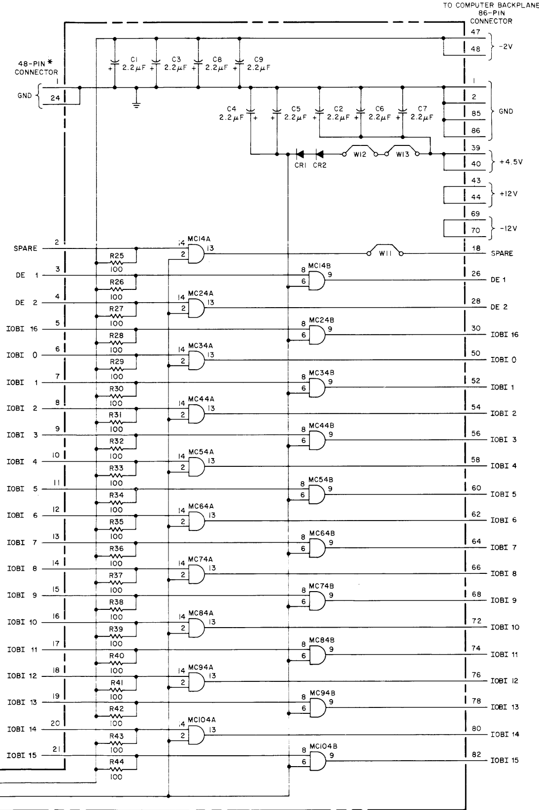
Figure 3-4. I/O-2 Extender Driver Card (02116-6183) Schematic Diagram
