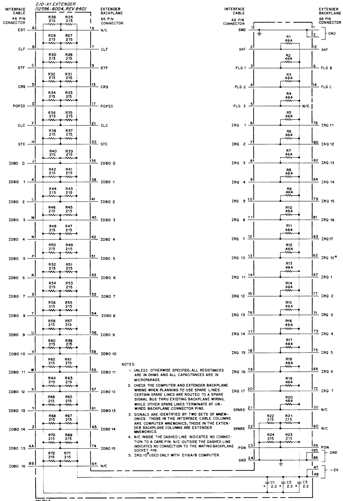
Figure 3-6. I/O-X1 Extender Card (12596-6004) Schematic Diagram
