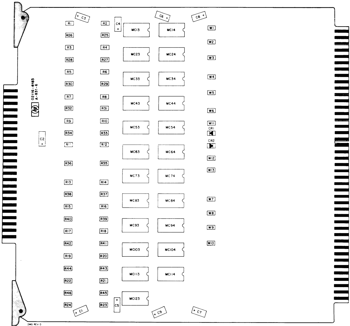
Figure 3-3. I/O-2 Extender Driver Card (02116-6183) Parts Location Diagram
