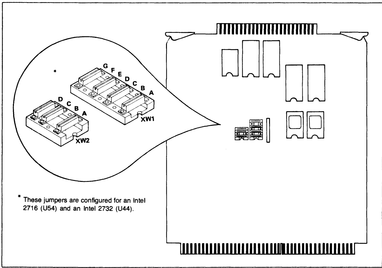
Fig. 2-2. ROM Configuration Jumper Positions
