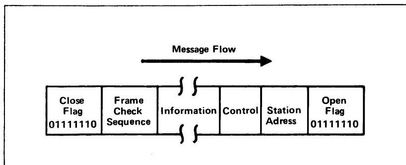
Figure 3-1. HDLC Frame Format
