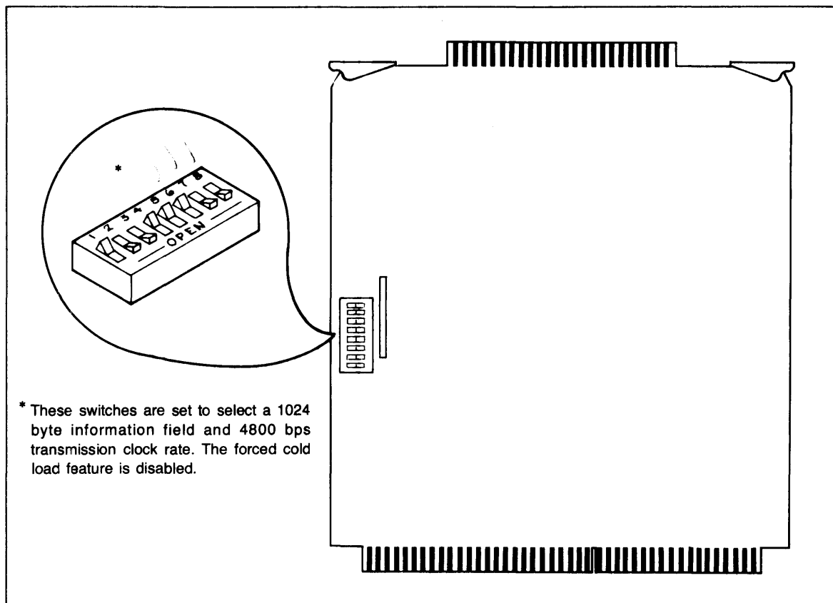
Figure 2-3. DIP Switch Position
