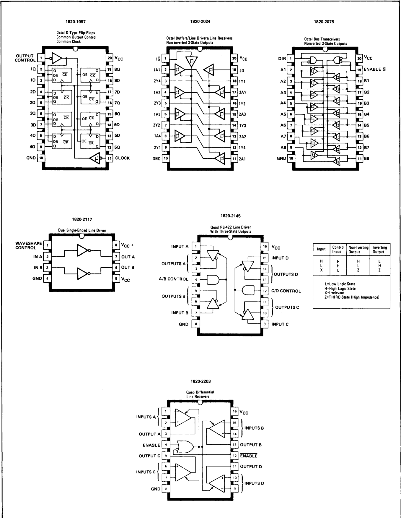
Figure 7-4. Integrated Circuit Base Diagrams (Continued)
