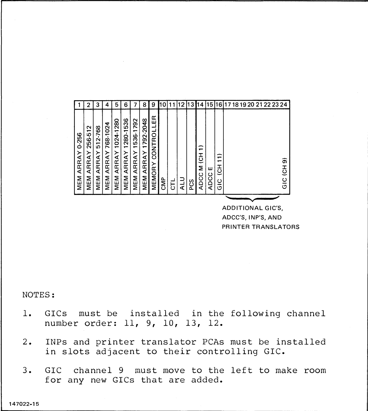
Figure 9. Series 44 Slot Locations (Single Card Cage Configuration)
