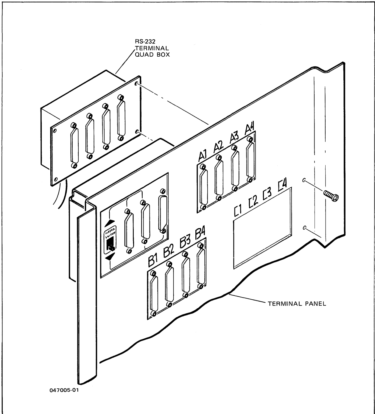
Figure 6. Series 33 Terminal Panel
