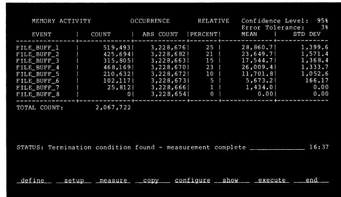
Figure 1. Memory Activity histogram (top) and the corresponding tabular form (bottom) showing file buffer usage during program execution.
