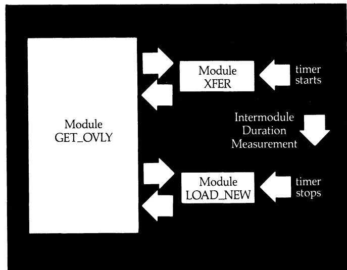
Figure 5. Diagram of an Intermodule Duration measurement from Module XFER to Module LOAD_NEW.
