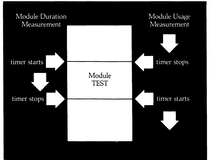
Figure 4. The Module Usage measurement is the complement of the Module Duration measurement.
