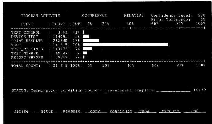
Figure 3. Program Activity measurement indicating that module TEST represents 70% of the overall system activity.
