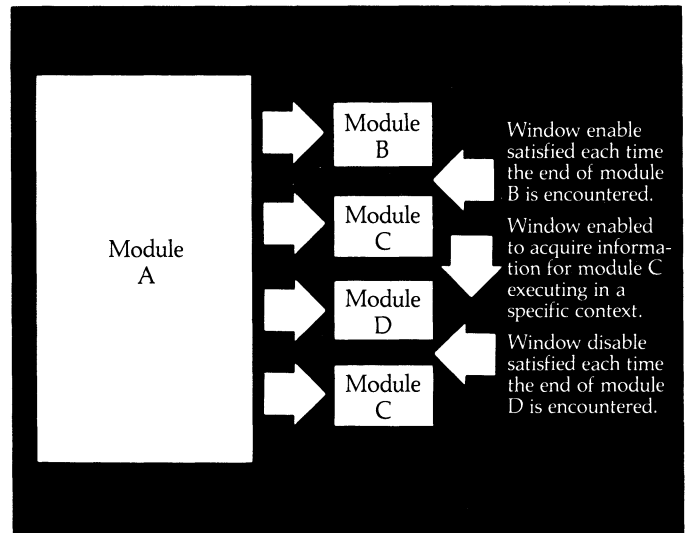
Figure 7. Execution of modules B and D can window data collection concerning module C. Note that module C executed again, but since the context requirements defined by the window specification were not met, no information was collected by the analyzer.
