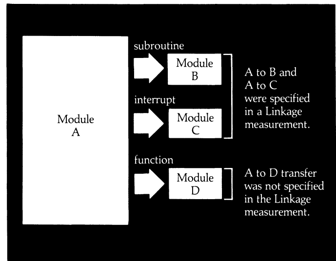
Figure 6. An Intermodule Linkage measurement specifying that transfers from module A to B and A to C are to be analyzed.
