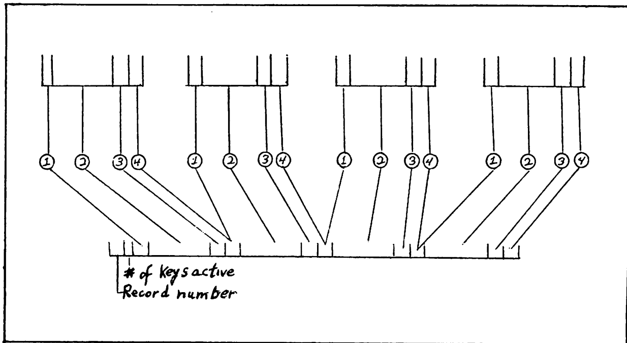
FIGURE 4. KEY ENTRY BLOCK. Words 1 & 2 contain the relative record number for this block. word 3 contains the number of active keys. Notice how items 4 and 1 are shared by adjacent KEY ENTRIES.
