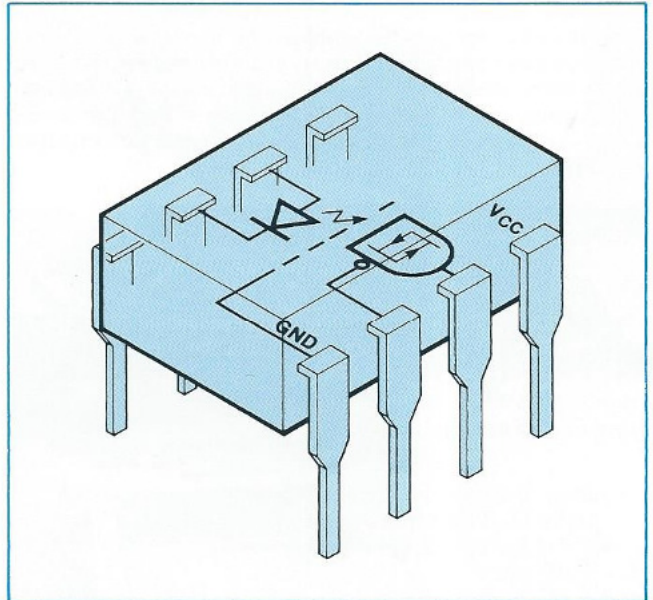
Sensitive enough to be driven by most CMOS circuitry, the HCPL-2200 Logic-Gate Optocoupler offers high speed and a wide range of V_{cc} capability.
