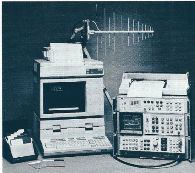
The new HP 85864A EMI Measurement Software program leads you through an EMI measurement from the setup to a final hard-copy plot of the test results. You do not need BASIC programming knowledge to use this software.
