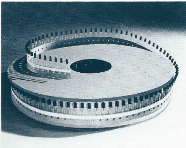
Two new tape and reel options for T-1 and T-1 3/4 LED lamps let you select either 5 mm or 2.54 mm spacing for use with automatic insertion equipment.
