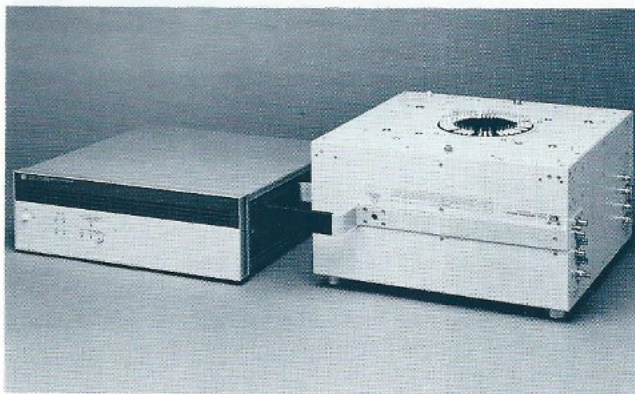
The HP 4085M Switching Matrix (at right) and its controller form a dedicated subsystem for use with the HP 4145A Semiconductor Parameter Analyzer.
