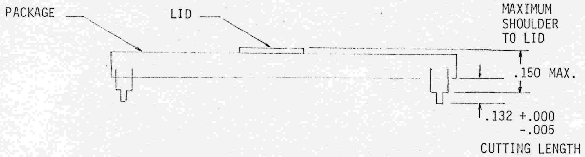
SIDE VIEW 42 LEAD CERAMIC PACKAGE H.P. PART #1260-0791 AND LID #1260-0618
