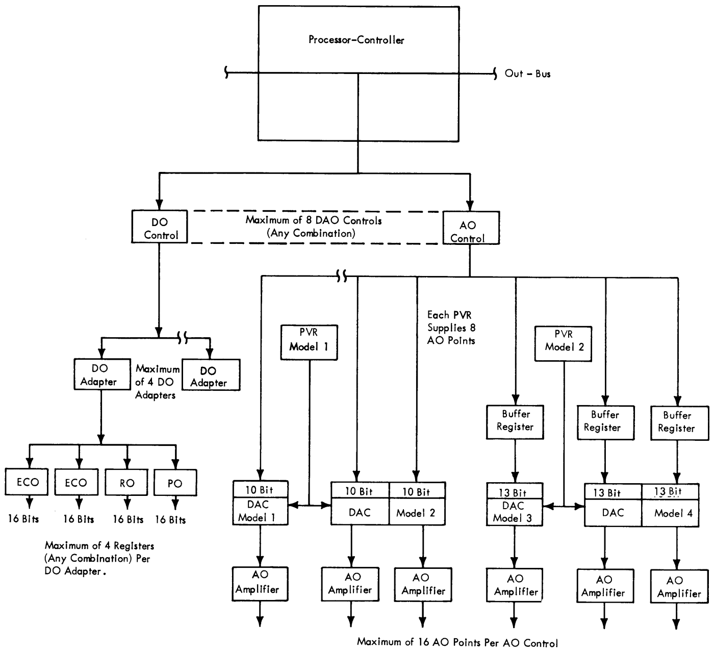
Figure 35. Schematic of Digital and Analog Output Features
