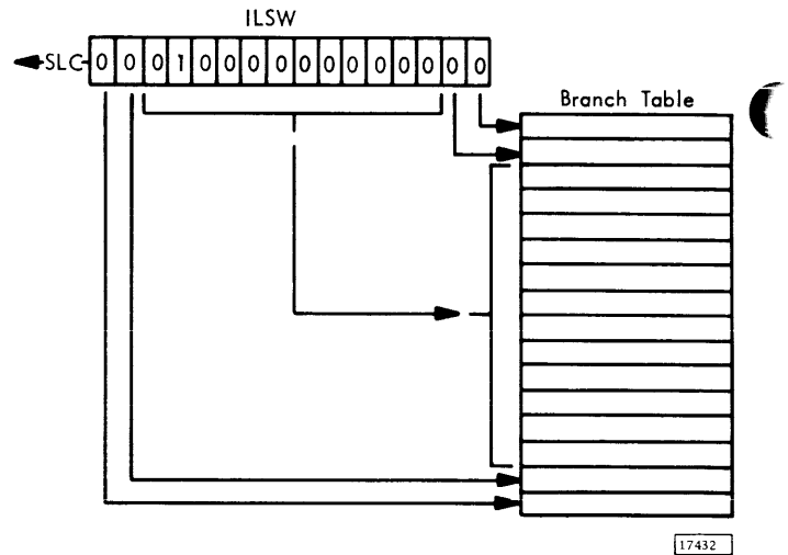
Figure 27. ILSW Branch Table
