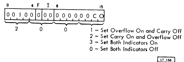
Figure 11. LDS Hexadecimal
