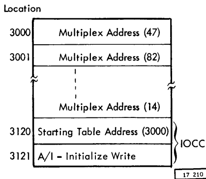
Figure 32. Multiplexer Address Table, Random Addressing
