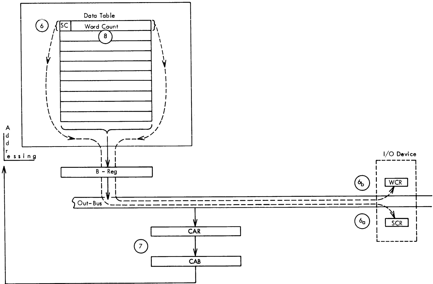
Figure 22. Data Channel Operation
