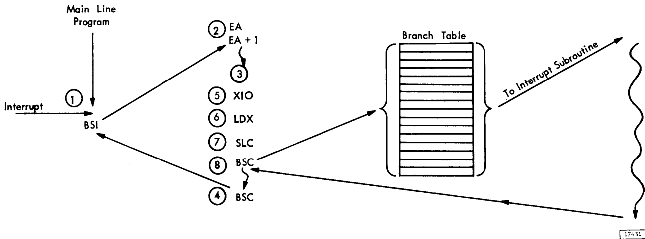
Figure 26. Program Identification of Interrupts
