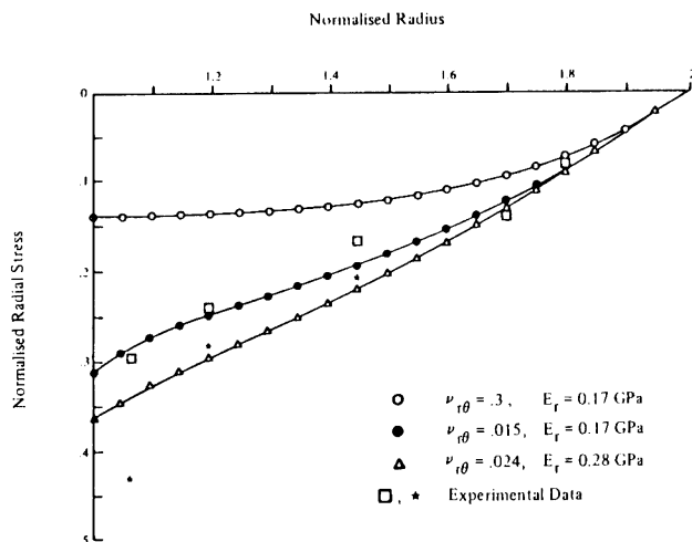
Fig. 3—Comparison of the theoretical and experimental radial stress in two experimental tape reels. Comparison of the effect of the value of Poisson's ratio \nu_{r\theta} on the predicted radial stress. The analysis uses \nu_{\theta r} = 0.3 and E_\theta = 3.45 GPa.
