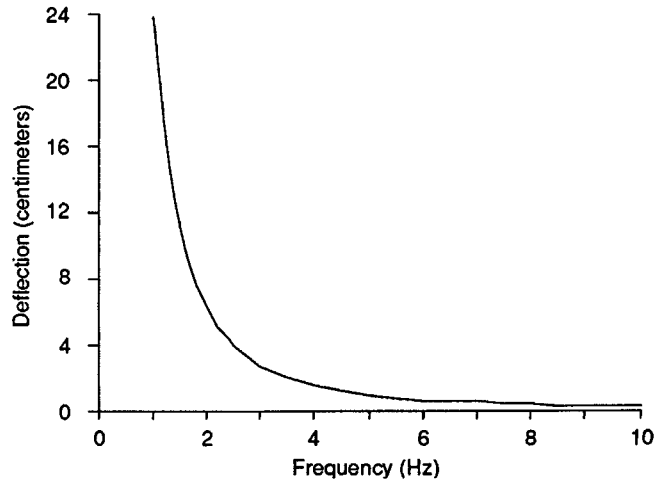
Figure 2: Deflection of a Single Beam under Gravity
