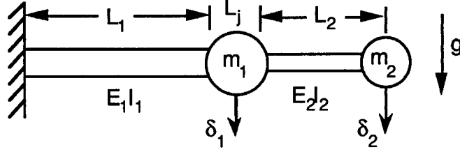
Figure 3: Two Cantilevered Beams with Masses
