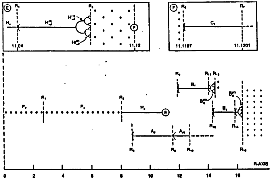
Figure 4: This diagram, reproduced from [5], is a manually-produced report similar to the diagrams that the Bifurcation Interpreter generates automatically.
