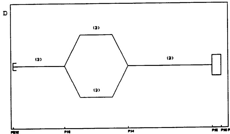
Figure 3: Expanding the interval from p = 5.6 to p = 10 shows details of the class D of order-3 orbits. Starting as a single family, the class splits into a pair near p = 6.7 and these merge again near p = 8 .
