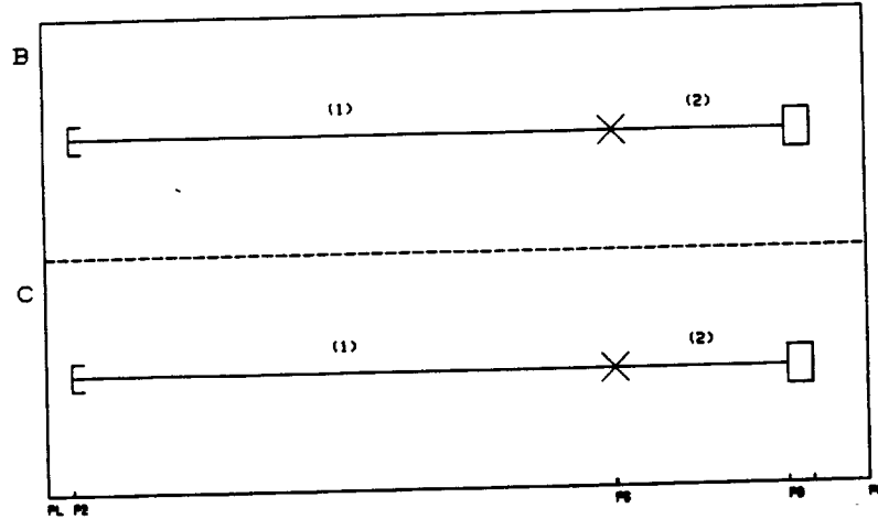
Figure 2: Expanding the interval from p = 3 to p = 5.7 shows details of classes B and C from figure 1. Each class begins as order 1, then doubles to order 2 via supercritical-flip bifurcations. Expanding the interval indicated by the rectangles would show further doubling. The Interpreter recognizes this progression as a period-doubling cascade, and reports it as such.
