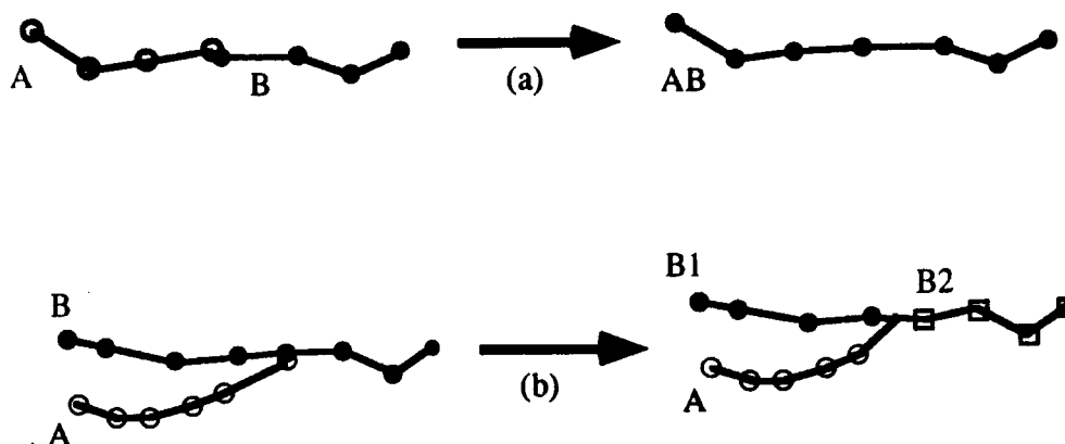
Figure 10: Merging families: (a) If family A extends to meet the first known instance of B , the two families are merged to form a single family AB . (b) If A coincides with a point in the middle of B (at a synchronization value of the parameter), B is split into two families B_1 and B_2 . A and B_1 vanish together at a bifurcation somewhere before the synchronization point, and B_2 appears there. Note that, in this figure, the horizontal direction represents the p -axis, while the vertical direction represents the location of the points in state space (projected onto a one-dimensional subset).
