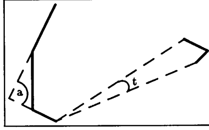
Figure 8: Two groups with a type_1 relationship. “t” represents the aspect the right group presents to the left. “a” is the angle of projection of the first group. The probability that the second group falls in the first’s projection is approximated by \frac{a-t}{2\pi} .
