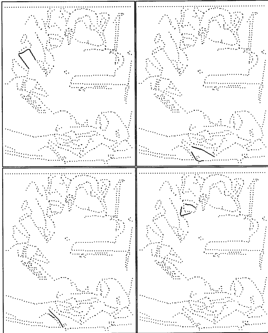
Figure 4: The second through fifth pairs of convex groups chosen by the grouping system, from the image in Figure 3. The groups on the left each come from a single object, the hammer and the phone cord. The group on the upper right has edges from the sandwich and phone cord. The edges in the lower right come from the folds and stripes of the sweater.
