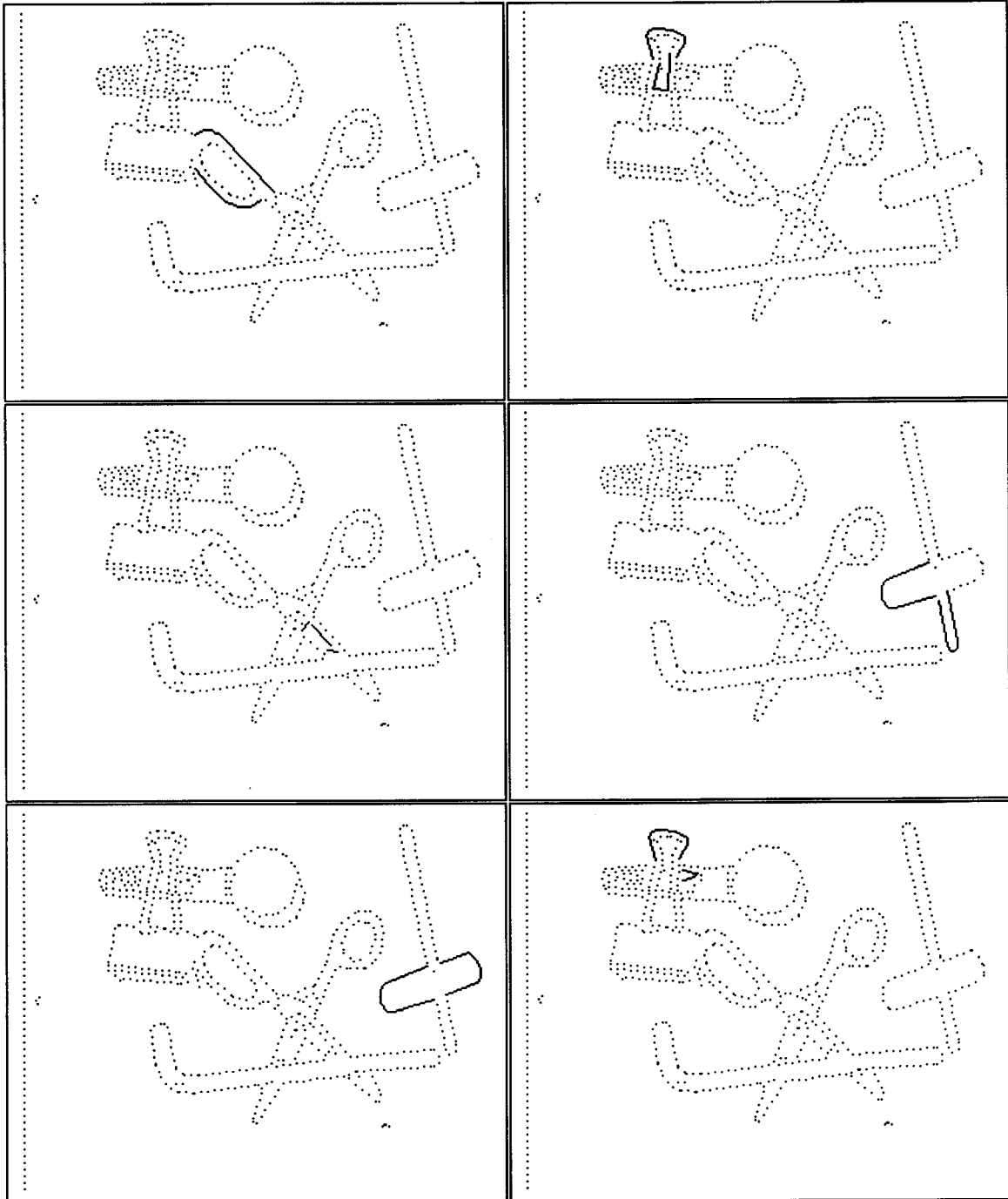
Figure 20: The second through seventh pairs of convex groups selected by the grouping system, from the picture in Figure 19. The second and sixth pairs are correct.
