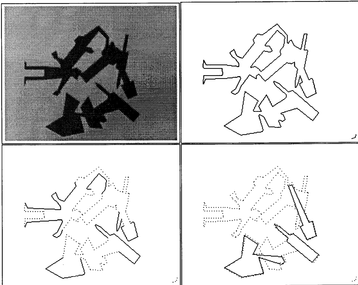
Figure 1: Recognition using grouping. In the upper left corner is a picture of objects cut out of paper. The upper right shows line approximations to the edges found in the image. The lower left shows the groups of convex edges found that contain four or more lines longer than ten pixels. The lower right shows the three objects found by indexing into a data base of sixteen objects (shown in Figure 13) using individual groups. Some big groups contain edges that all come from a single object, but do not lead directly to the recognition of that object. That may be because those edges do not provide enough information or contain edges detected with too much error. (continued in Figure 2.)
