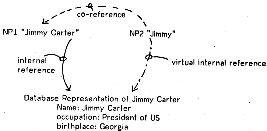
Fig. 1. Reference Links Between Noun Phrases
