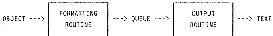
Figure 1: Architecture of the basic pretty printing algorithm.
