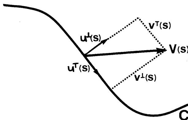
Figure 7. The decomposition of velocity V(s) into tangential and perpendicular components
