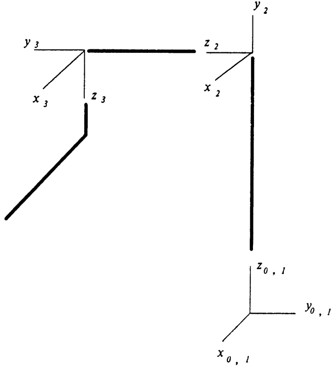
Figure 3: The link coordinate system.
