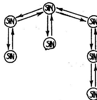
Figure 3 - Flow of Control and Subproblems in SIN When Problem is a Sum of Three Terms
