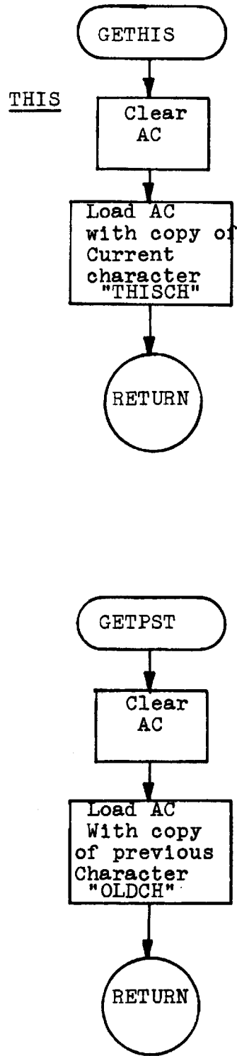
FIGURE E-4. The GETHIS and GETPST Routines
