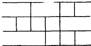
Figure 1.3.1 Sorting network.
