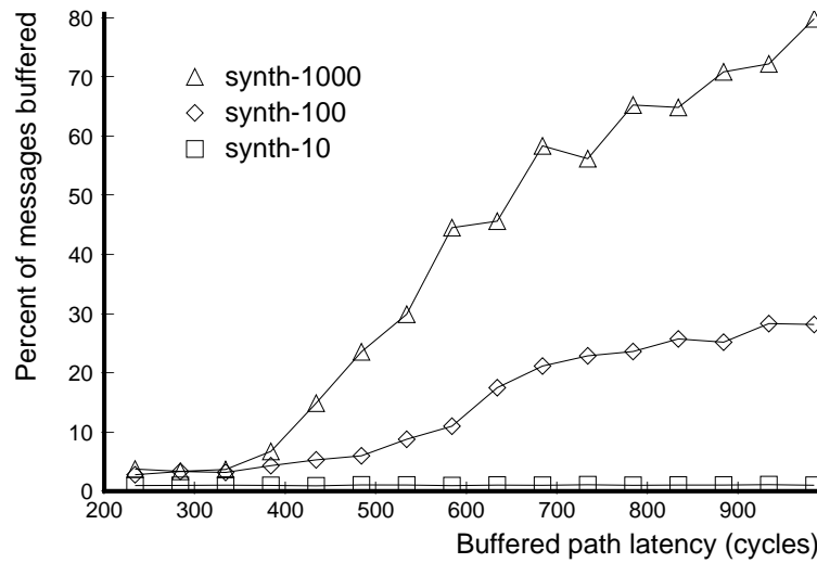
Figure 7-22. Fraction of messages buffered versus cost of the buffered path given T_{\text{interhandler}}=275 cycles (four processors).
