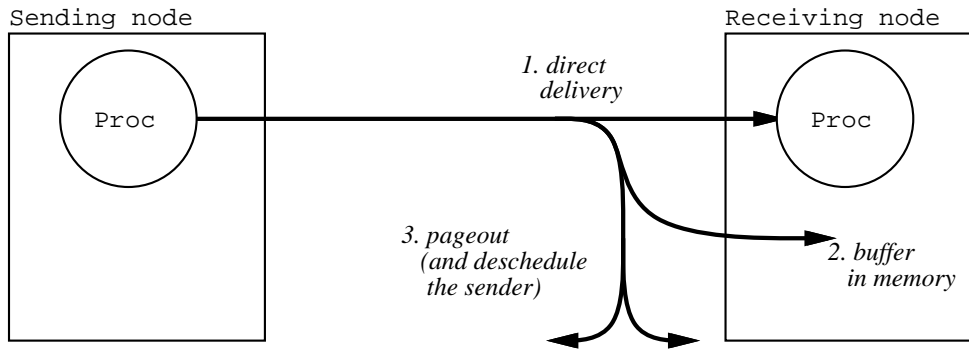
Figure 5-2. There are three message reception cases. In the fast case, (1), messages are received directly by the processor. In the ordinary buffering case, (2), messages are buffered by software in memory, but the memory is physical memory that is resident on the node. In the worst case, (3), a node can continue to receive messages while simultaneously paging out message buffers. A reserved second network is used to assure that paging can proceed without deadlock in the worst case as well as for the overflow control mechanism that helps avoid paging.
