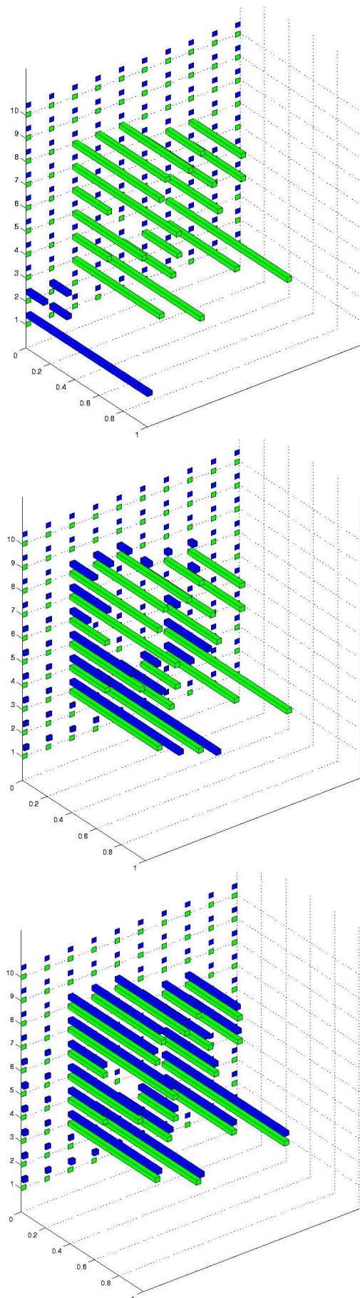
Fig. 8. Simulation results show the actual (dark) and target (light) distribution of PN s over \mathcal{H} , at the end of various rounds: the first round (top), at T_{out} (middle), and at T_{stab} (bottom).
