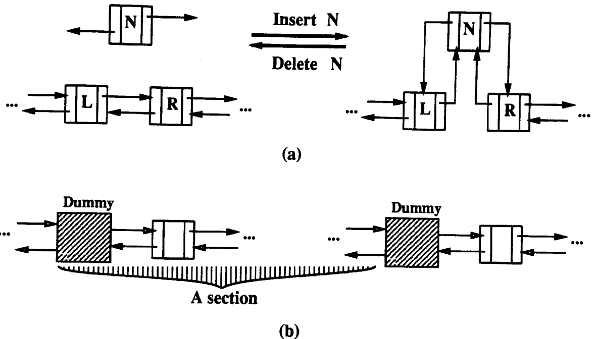
Figure 3.1: Concurrent insertion on DLL
