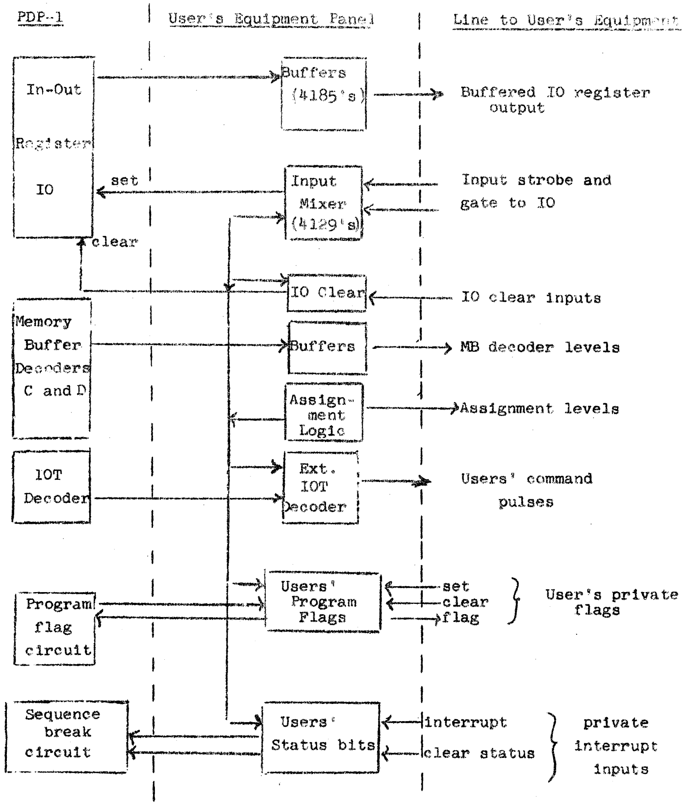
Figure 4 -- Users' External Equipment Panel
