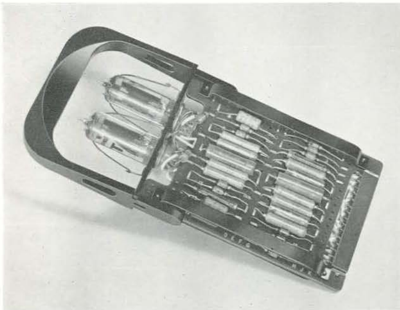
Typical plug-in unit from STANTEC-ZEBRA.
