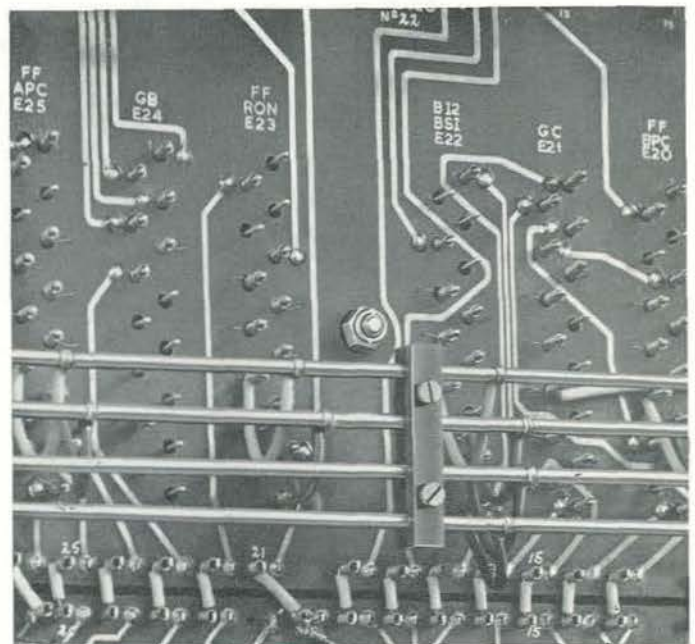
Close-up of a section of STANTEC-ZEBRA printed circuit showing wrapped-joint technique at terminals.
