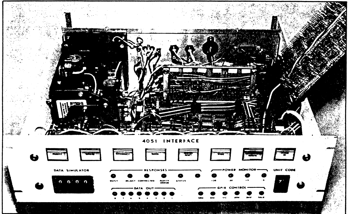
The Front Panel of the CDC 3200—4051 Interface showing indicator lights and thumbwheel switches. Both GPIB and CDC responses are shown by the lights.
