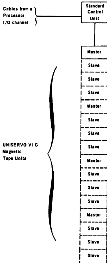
Figure 2-1. Non-Simultaneous Operation Subsystem Configuration, Block Diagram
