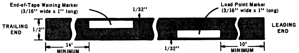
Figure 4-10. Tape Markers
