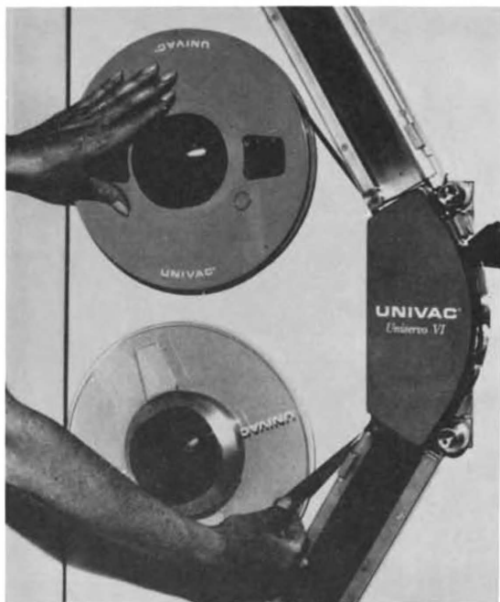
Figure 4-8. Tape Threaded Over Lower Vacuum Column
