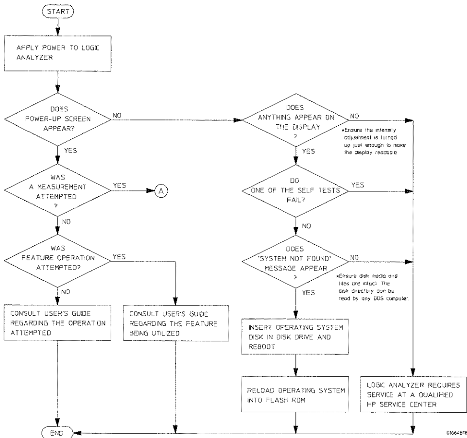
Troubleshooting Flowchart 1
