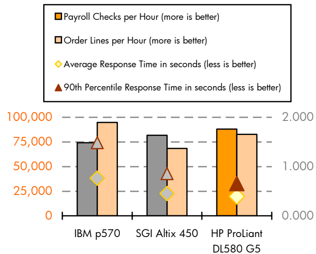
Figure 1. HP ProLiant DL580 G5 OASB Medium Model performance comparison with IBM and SGI platforms
