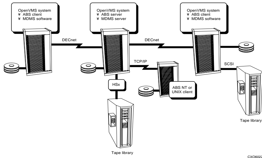
Figure 2–1 Recommended Installation
