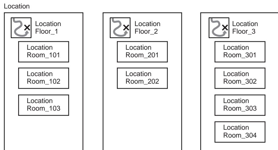
Figure 17–6 Named Locations
