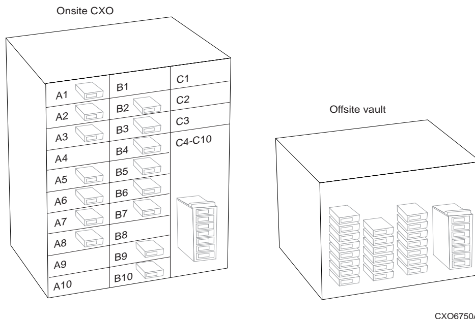
Figure 17–5 Volume Locations
