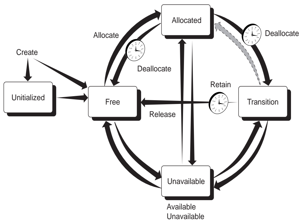
Figure 20–1 Volume States
