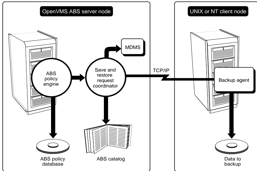
Figure 2–2 ABS UNIX or NT Client Configuration
