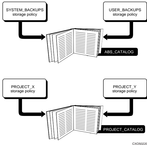
Figure 1–3 ABS Catalogs
