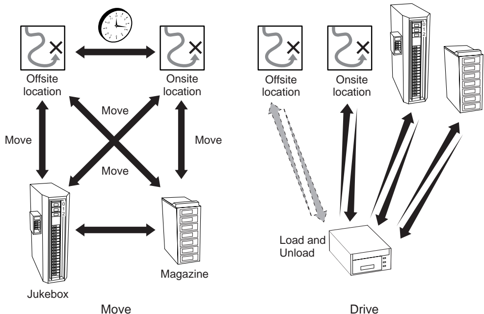
Figure 21–2 Volume Rotation
